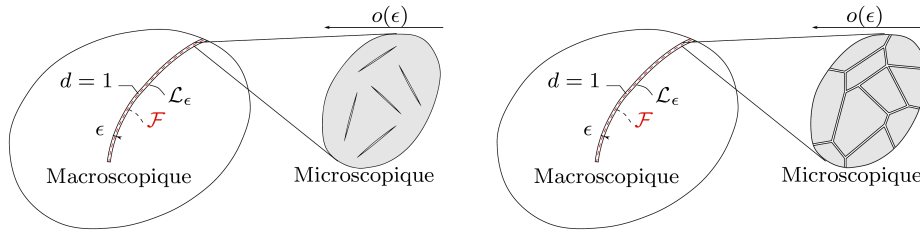
Fig. 2 On the left : The transitory state toward full damage. On the right : 3D representation of a macroscopic crack as a layer of thickness \epsilon of a fully damaged material.
