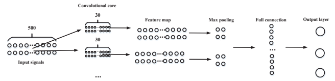
Figure 10 CNN structure
