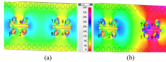
FIGURE 2. Two different slot array configurations with single and double excitation with their phase distribution at 26.75 GHz, for: (a) \Delta\phi = 0^\circ , (b) \Delta\phi = 225^\circ .
