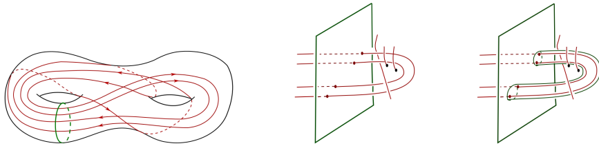
FIGURE 2 – The vertical surface S (in the middle) over the green curve is a torus with four boundary components. By replacing these four boundary components by a handle, one obtained a genus 2 closed surface S' (right picture) and |\chi(S')| < |\chi(S)| .
