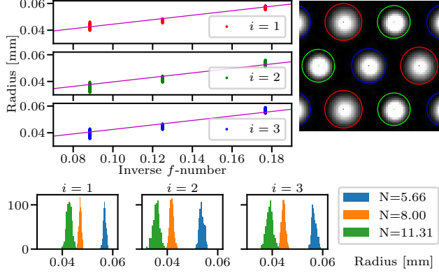
Figure 5: Micro-image radii as function of the inverse f -number with the estimated lines (in magenta). Each type of micro-lens is identified by its color (type (1) in red, type (2) in green and type (3) in blue) with its computed radius. For each type an histogram of the radii distribution is given.
