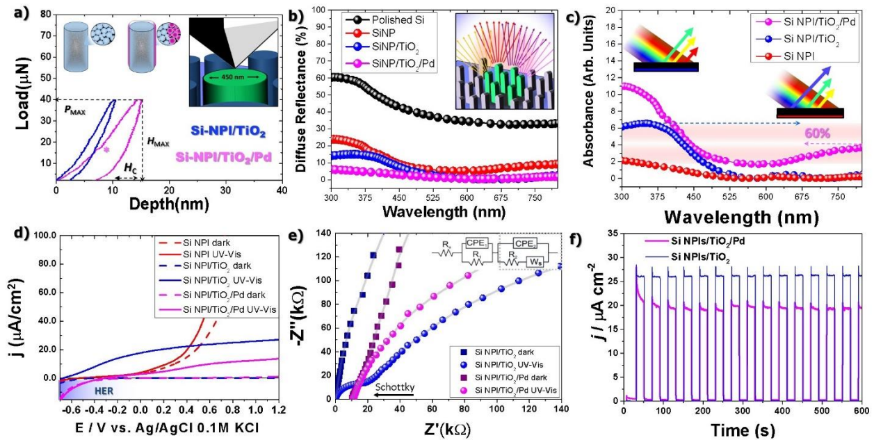
Figure 2: a) low-load indentation experiments on single pillars, H_{\max} , P_{\max} and H_c show the maximum penetration, maximum load and residual imprint respectively. Insets show diagrams of the structure and indentation experiments b) Diffusive reflectance spectra of the samples c) Absorbance spectra of the prepared samples, insets show schematics of the absorption. Dashed lines are a guide to eye pointing to the IR enhanced response that corresponds to ~60% of the UV absorption of bare \text{TiO}_2 samples. d) Linear voltammetry curves recorded for all the samples, dashed lines correspond to dark conditions while full lines to illuminated conditions. Blue shaded region corresponds to the negative potentials where hydrogen evolution reaction takes place. e) Nyquist plots of the \text{TiO}_2 and Pd/ \text{TiO}_2 coated samples. Lines shows the response in illuminated conditions (●) and in dark conditions (■). Gray faded lines are the fitted curves. Inset shows the circuit model used for fitting the data. f) Chronoamperometric response of \text{TiO}_2 and Pd/ \text{TiO}_2 samples during multiple light on/off cycles collected at +1 V vs. ag/AgCl/0.1M KCl.
