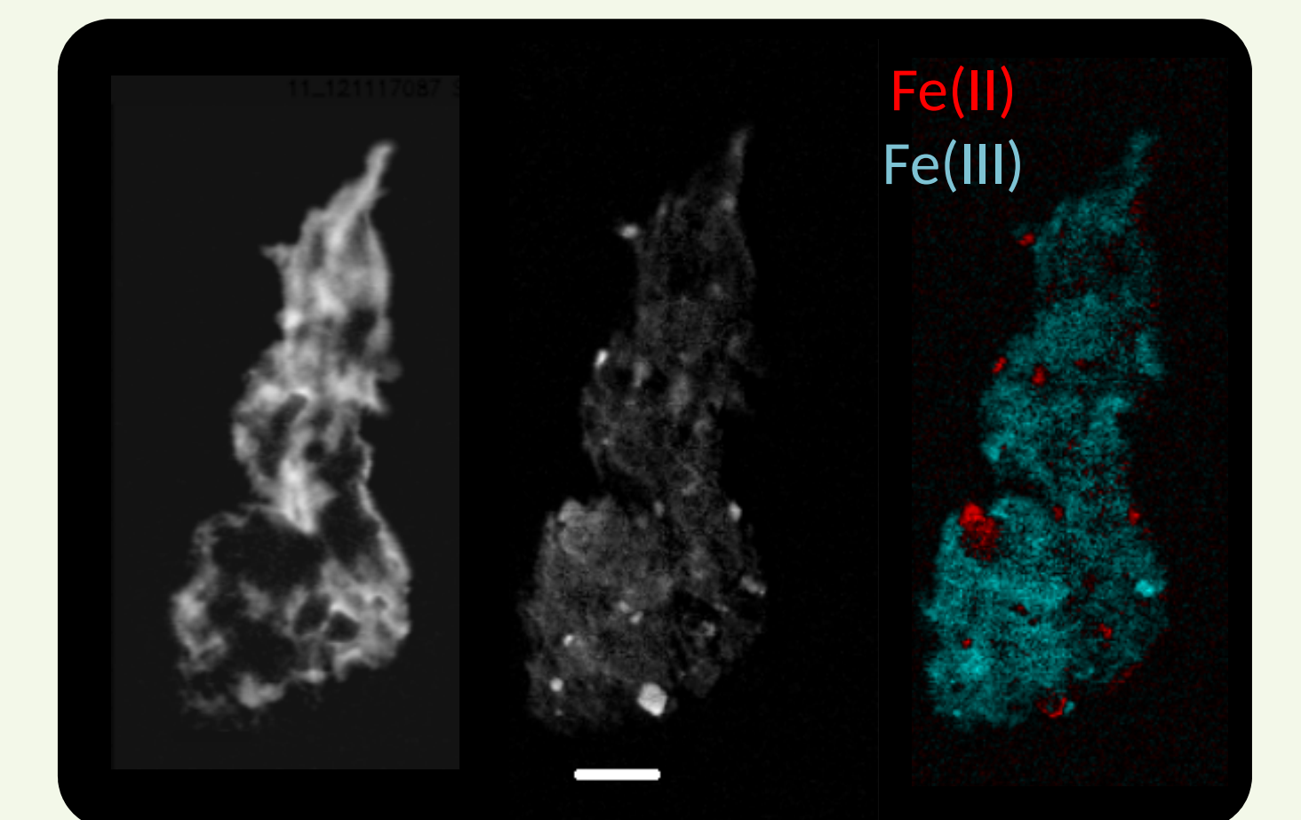
STXM analysis of a reduced particle (< 53 μm fraction) C map (left), Fe map (middle), Fe speciation map (right)
