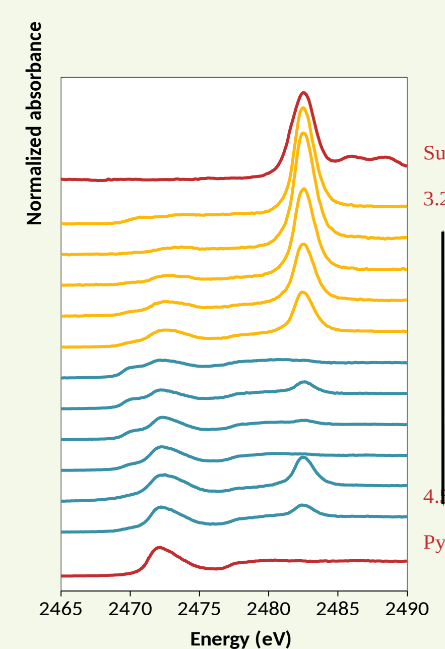
S K-edge XANES of natural sediments
