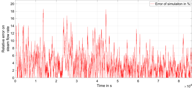
Fig. 6. Relative error between the model and the measured values for the steam flow
