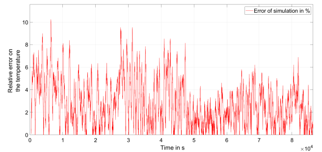
Fig. 5. Relative error between the model and the measured values for the temperature
