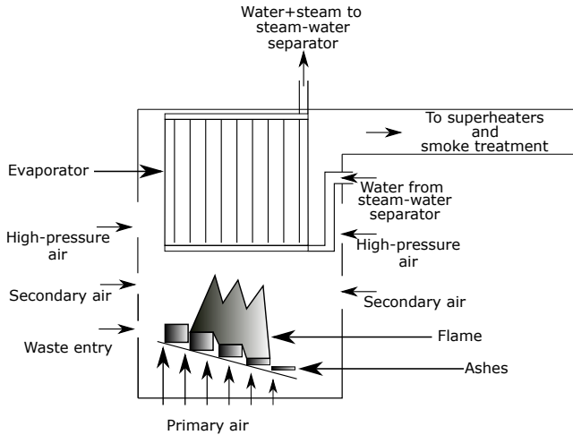
Fig. 1. Configuration of the incinerator
