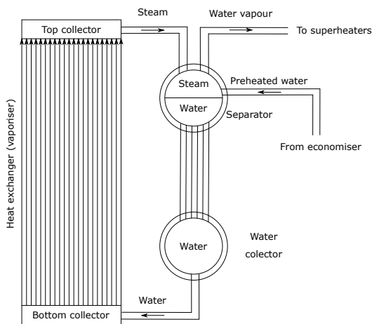
Fig. 2. Boiler: water vapour separator
