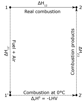
Fig. 4. Combustion cycle
