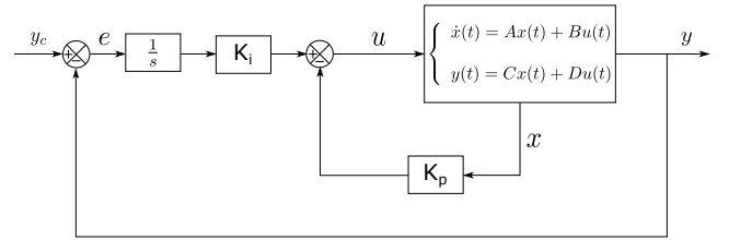
Fig. 7. Full-state feedback with integral loop
