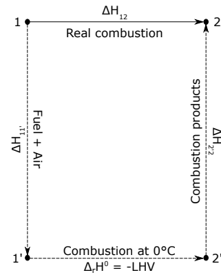
Fig. 4. Combustion cycle
