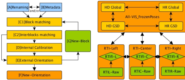
Figure 5: Diagram of the iterative pipeline processing.
