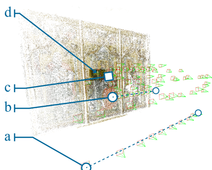
Figure 3: Multidimensionnal blocks merged : global (a) and close-up (b) photogrammetry, multistereo H-RTI (c) and multitemporal/multispectral Technical Photography (d) on Venasque case-study.
