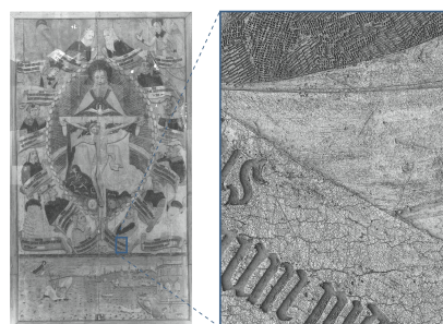
Figure 4: Orthophotographic shaded relief map of the high resolution multi-focal photogrammetric survey with HD and HR sensors on Trinité case-study.
