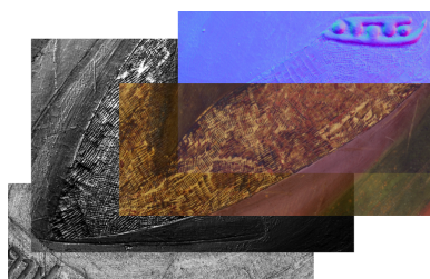
Figure 2: Blended view of orthophotographic shaded relief map, specular H-RTI, VIS photograph and normal map.
