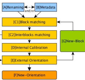
Figure 5: Diagram of the iterative pipeline processing.
