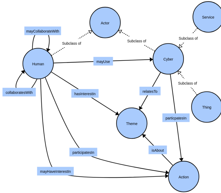
Fig. 2. The network ontology modeled using WebVOWL [27].
