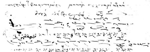
Fig. 23 Detail from the transcription by Petros Peloponnēsios of pistrifi tō kantemira makâm sultanî arâk ûsûl devri k[e]bîr – from Gritsanis Ms. 3, f° 14 r°. 186
