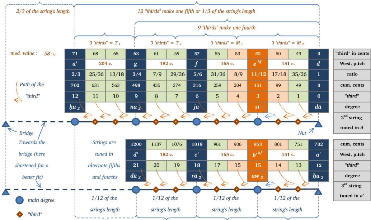
FHT 7 Scale of the pseudo-Şafadi in the hypothesis of an equal-strings division on a tumbūr tuned in alternate fifths and fourths.
