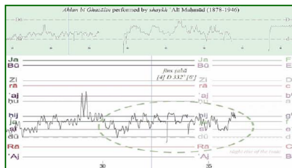
Fig. 97 Two frames from the video-animated analysis of Ahlan bi-Ghazālīn performed by sheikh 'Alī Maḥmūd. 398
