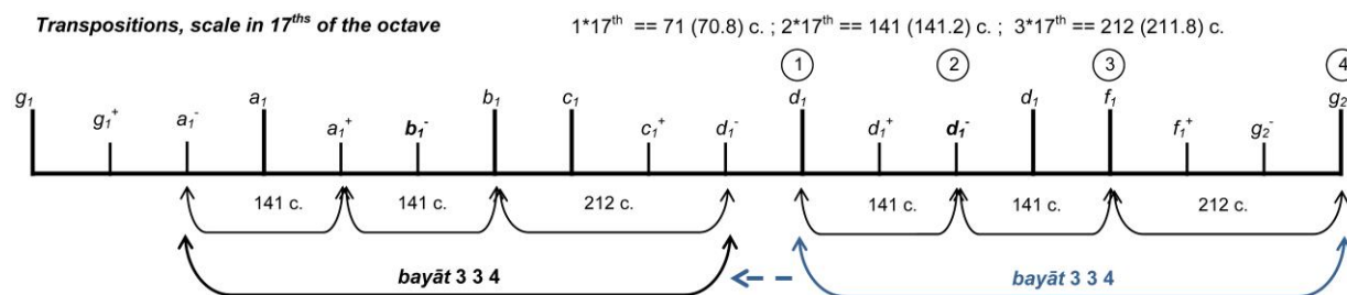
FHT 35 Example of a transposition of the same tetrachord as in FHT 34 on a 17 th of the octave grid from d to a . All transpositions in this equal-temperament grid give similar intervals.
