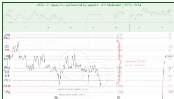
Fig. 99 Frame from the video-animated analysis of Ahlan bi-Ghazālīn performed by sheikh 'Alī Maḥmūd, showing the effective use of the non-octavial scale (from dū = d to Zi = D^b ) of maqām Ṣabā .
