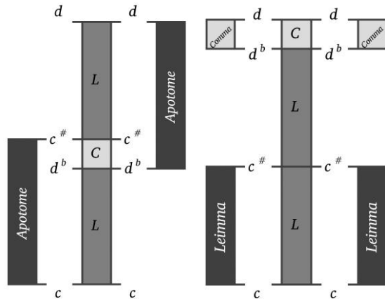
Fig. 51 To the left: Accidentals in Pythagorean theories adapted to the Common practice scale of western music are divisive: intervals c_c c^{\#} and d d^{\flat} intersect. To the right: Conjunct intervals and consecutive action of the accidentals with Urmawī: intervals c_c c^{\#} and d d^{\flat} are independent from one another, and separated by c^{\#} d^{\flat} which is one leimma . 258
