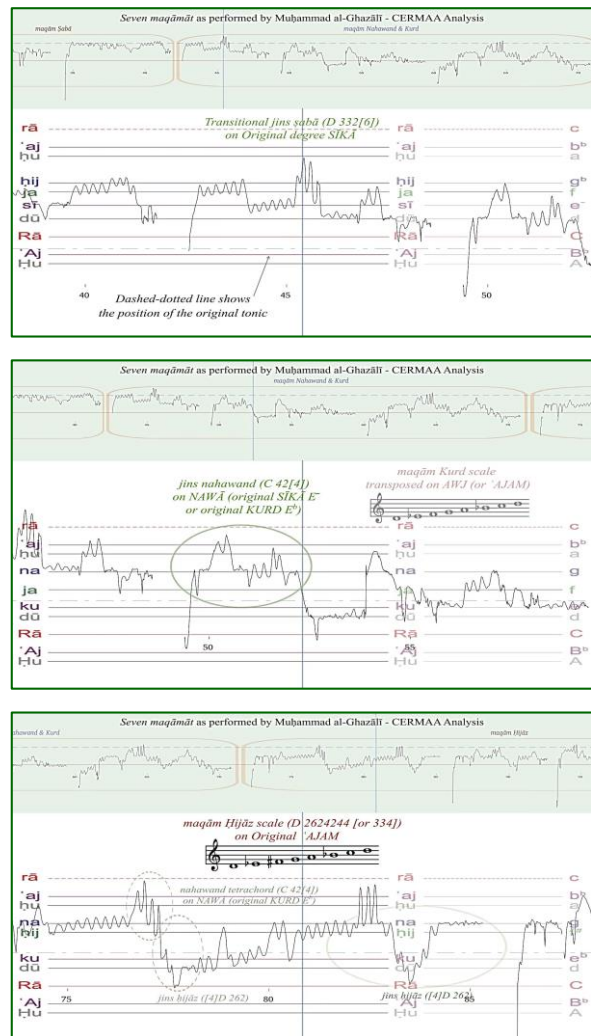
Fig. 95 Three frames from the video-animated analysis of 7 maqāmāt as performed by the qārī 393 Muḥammad al-Ghazālī. 393
