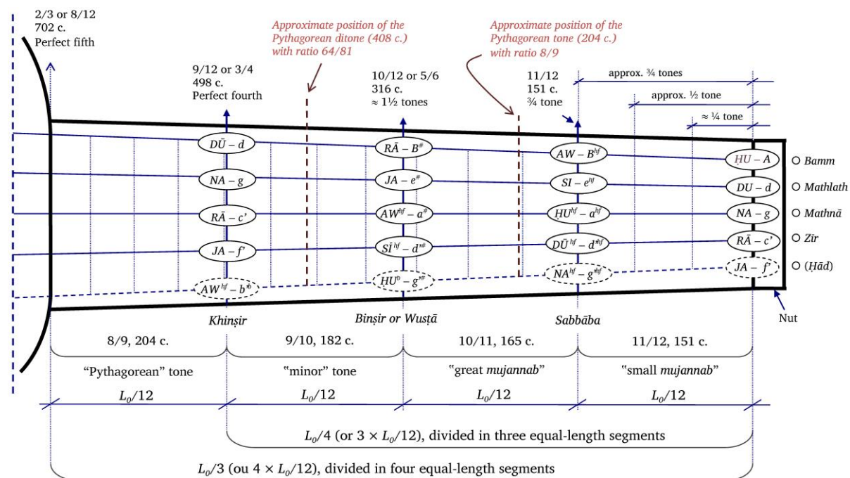
FHT 3 Division of the fingerboard of the ‘ūd on a 12 equal string-parts basis using the solmization proposed by the author. “ hf ” stands for “half-flat” – adapted from [Beyhom, 2012, p. 72 (Fig. 14)].
