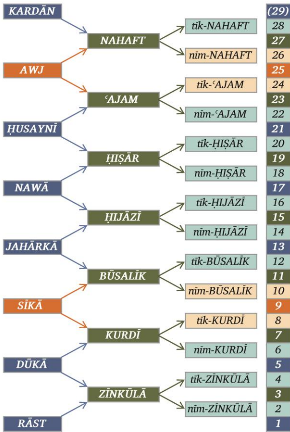
Fig. 29 The 28 “quarter-tones” (“maqāmāt” = pl. of maqām) of Shihāb-a-d-Din divided into burdāt , arabāt , tikāt and nīmāt . 217
