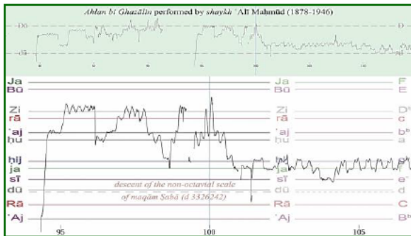
Fig. 104 Frame from the video-animated analysis of Ahlān bi-Ghazālīn performed by sheikh ‘Alī Maḥmūd. 406
