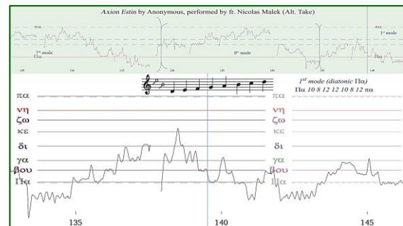
Fig. 85 One frame (top) to the end of the 7 th Byzantine mode in the video-animated analysis of Axion Estin performed by fr. Nicolas Malek, and one frame (bottom) towards the end of the analysis of the second (alternate) take. 361
