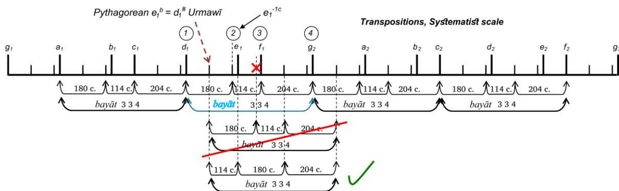
FHT 34 Theoretical transposition in the “Systematist scale” of a bayāt tetrachord [d ↑3 3 4], or M_1 M_2 T ( mujannab 1 mujannab 2 whole-tone) on the degrees g , a and e^b : the transposition on d^\# enforces the inversion of the mujannab (s) (“neutral seconds”) as M_2 M_1 T .
