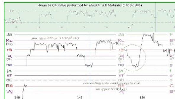
Fig. 107 Frame from the video-animated analysis of Ahlān bi-Ghazālīn performed by sheikh ‘Alī Maḥmūd, showing the leap of near-octave between Rā = C and ‘aj = b^b and the descending nahawand arpeggio between 148 s_a and 150 s_a.
