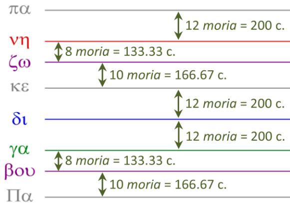
Fig. 69 Graphic scale of the 1 st Byzantine mode (“diatonic”) – used in the video-animated analyses, with the theoretical values of intervals (2 nd Reform of 1881) given in “minutes” (“ moria ”) and cents. 328
