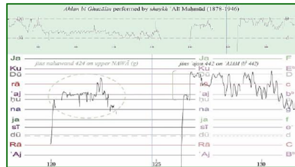
Fig. 106 Frame from the video-animated analysis of Ahlān bi-Ghazālīn performed by sheikh ‘Alī Maḥmūd, showing the beginning of the process of back and forths between jins nahawand 424 on na = g and jins ‘ajam 442 on ‘aj = b^b .
