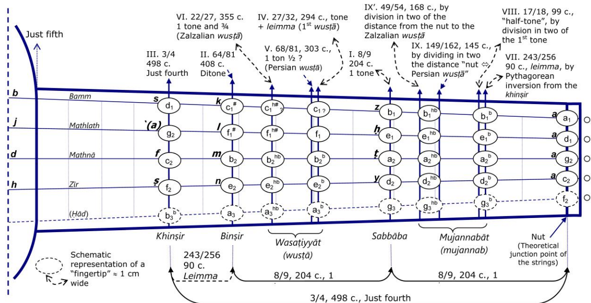
FHT 2 Fārābī’s sequential construction in the Kitāb al-Mūsīqī al-Kabīr of the meshing of the fingerboard of the ‘ūd using the Abjad alphabet (bold letters) for key notes – “ hb ” and “ hb ” are, respectively, “half-sharp” and “half-flat” accidentals in approximate quarter-tones. The column of letters to the utmost left corresponds to the junctions of the strings with the tailpiece, the right column (bold “ a ”) reminds that the strings make their (theoretical) junction on the nut; the fifth ( Hād ) string is theoretical – adapted and translated from [Beyhom, 2010c, v. 1, p. 205 (Figure 75)].
