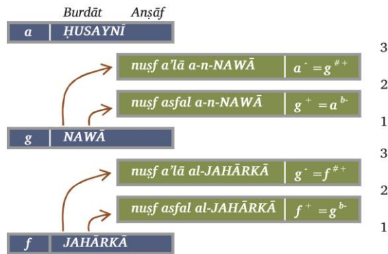
Fig. 9 Two upper anṣāf possible divisions (1) of the intervals in [Şafadī (a-Ş-), 1991]. 145
