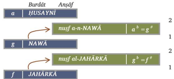
Fig. 8 Most probable division of the intervals in the A-sh-Shajara treatise. (Contemporary note names for the Arabic scale and western equivalents are provided in FHT 8: 211.) 139
