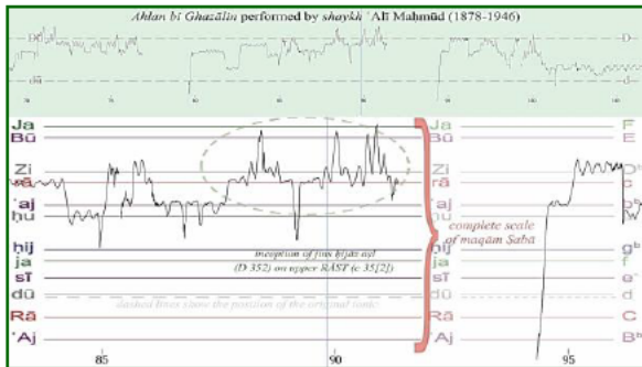
Fig. 103 Frame from the video-animated analysis of Ahlān bi-Ghazālīn performed by sheikh ‘Alī Maḥmūd, showing the complete scale of maqām Šabā . 405
