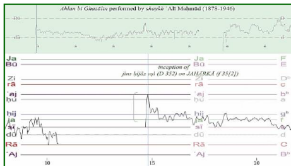
Fig. 96 Two frames from the video-animated analysis of Ahlan bi-Ghazālīn performed by sheikh 'Alī Maḥmūd, showing the initial jins šabā followed by jins hijāz on ja = f .
