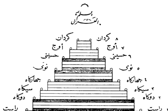
Fig. 28 The scale of “Arabian” [ maqām Rāst ] music according to Kāmil al-Khula’ī with whole-tone and three-quarter-tones intervals. 215
