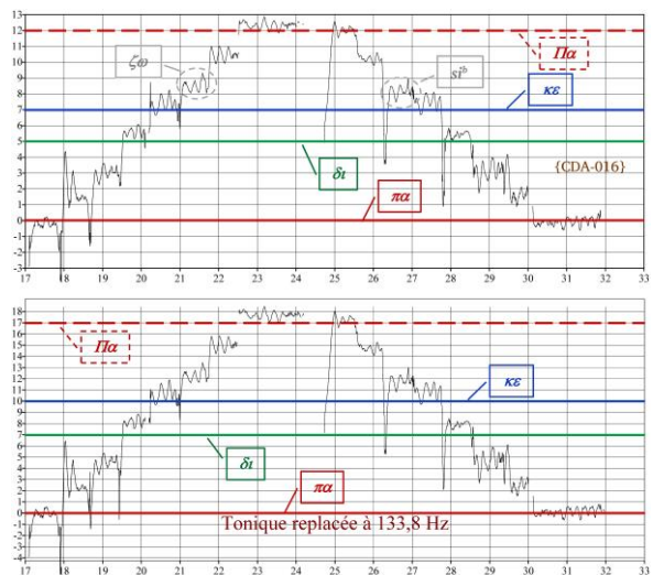
Fig. 61 Annotated (in French and Greek names of notes) example of scale analysis (1 st “Diatonic” mode of Byzantine chant performed by fr. Makarios Haidamous) with Praat – taken from [Beyhom, 2015, p. 333, Figure 263]. Above: Semi-tone (vertical axis) / time (in seconds – horizontal axis) grid drawn with Praat; below: 17 th of the octave (vertical axis) / time (in seconds – horizontal axis) grid. 295
