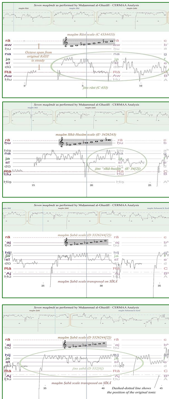
Fig. 94 Four frames from the video-animated analysis of 7 maqāmāt as performed by the qārī 393 Muḥammad al-Ghazālī.
