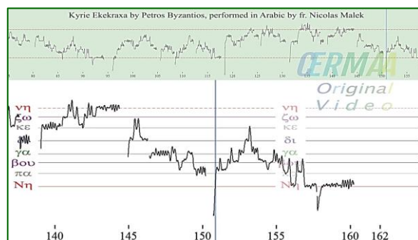
Fig. 73 Beginning and ending tonics in fr. Nicolas Malek’s interpretation of Kyrie Ekekraxa by Petros Byzantios in the Arabic version.
