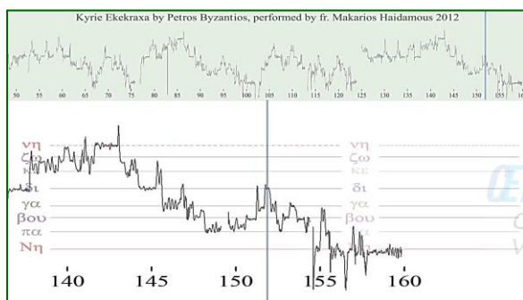
Fig. 72 Beginning and ending tonics in fr. Haidamou’s interpretation of Kyrie Ekekraxa (Arabic version). 334
