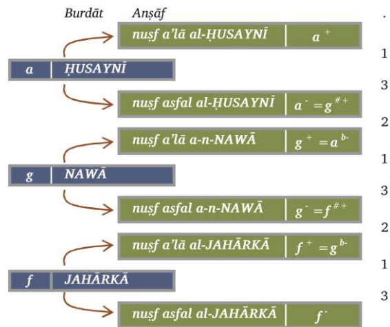
Fig. 10 Two upper anṣāf possible divisions (2) of the intervals in [Şafadī (a-Ş-), 1991].
