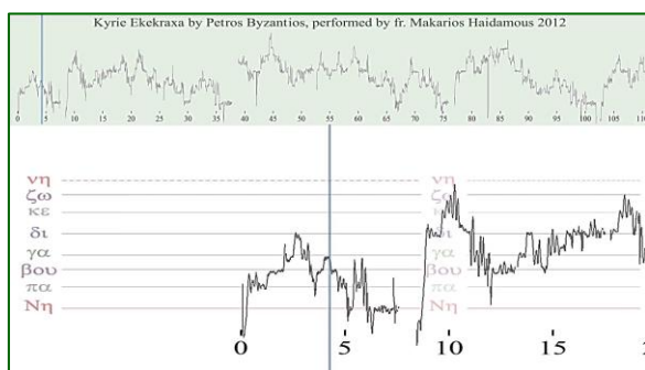
Fig. 71 Graphic scale of the 2 nd Byzantine mode – used in the video-animated analyses, with the theoretical values of intervals (2 nd Reform of 1881) in “minutes” (“moria”) and cents. (1 “moria” = 1200 c / 72 = 200 c / 12 = 16.67 c)
