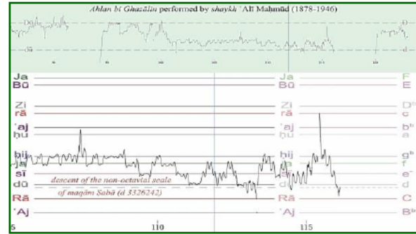
Fig. 105 Frame from the video-animated analysis of Ahlān bi-Ghazālīn performed by sheikh ‘Alī Maḥmūd, showing the continuation of the complete descent of the scale till the tonic dū = d with the closing jins šabā .
