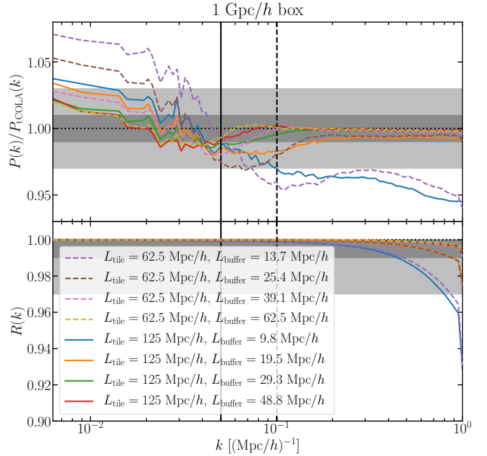
Fig. 6. Same as Fig. 5, but in a 1 \text{ Gpc } h^{-1} box containing 1024^3 particles.
