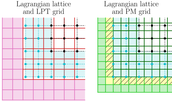
Fig. 2. Illustration of the different grids used within sCOLA. The Lagrangian lattice is represented by dashed lines. For each tile, central particles (in black) are surrounded by buffer particles (in cyan), which are ignored at the end of the evolution. The corresponding buffer region in other grids is represented in cyan. The left panel represents the “LPT grid” on which Lagrangian potentials \tilde{\phi}^{(1)} and \tilde{\phi}^{(2)} are defined. The central region has N_{\text{sCOLA}}^3 grid points (in red) and is padded by 2N_{\text{ghost}} cells in each direction (pink region). The right panel shows the “PM grid” on which the density contrast \delta^{\text{sCOLA}} , the gravitational potential \Phi^{\text{sCOLA}} , and the accelerations -\nabla_x^{\text{sCOLA}}\Phi^{\text{sCOLA}} are defined. The density contrast is defined only in the central region (which has N_g^3 grid points, in dark green). The gravitational potential is padded by 2N_{\text{ghost}} cells in each direction (light green and yellow regions), and the gridded accelerations only by N_{\text{ghost}} cells in each direction (yellow region). Solving the Poisson equation requires Dirichlet boundary conditions in six layers of N_{\text{ghost}} cells, denoted as hatched regions. For simplicity of representation, we have used here N_{\text{ghost}} = 1 .
