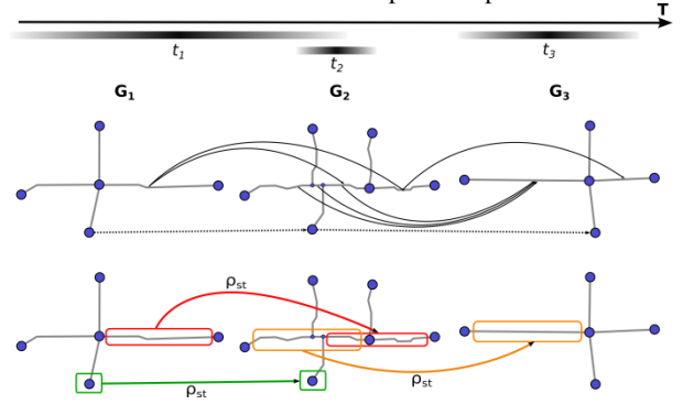
Figure 3: examples of matching links and spatio-temporal relations between elements of the temporal snapshots.
