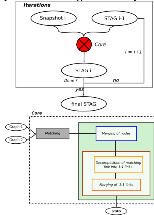
Figure 8: Global iterative approach for building the STAG.
