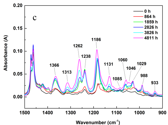
FIGURE 5. FTIR spectra of the outer surface of the insulating layer (a) between 3500 and 3800 \text{cm}^{-1} , (b) 1600 and 1850 \text{cm}^{-1} and (c) 900 and 1500 \text{cm}^{-1} .
