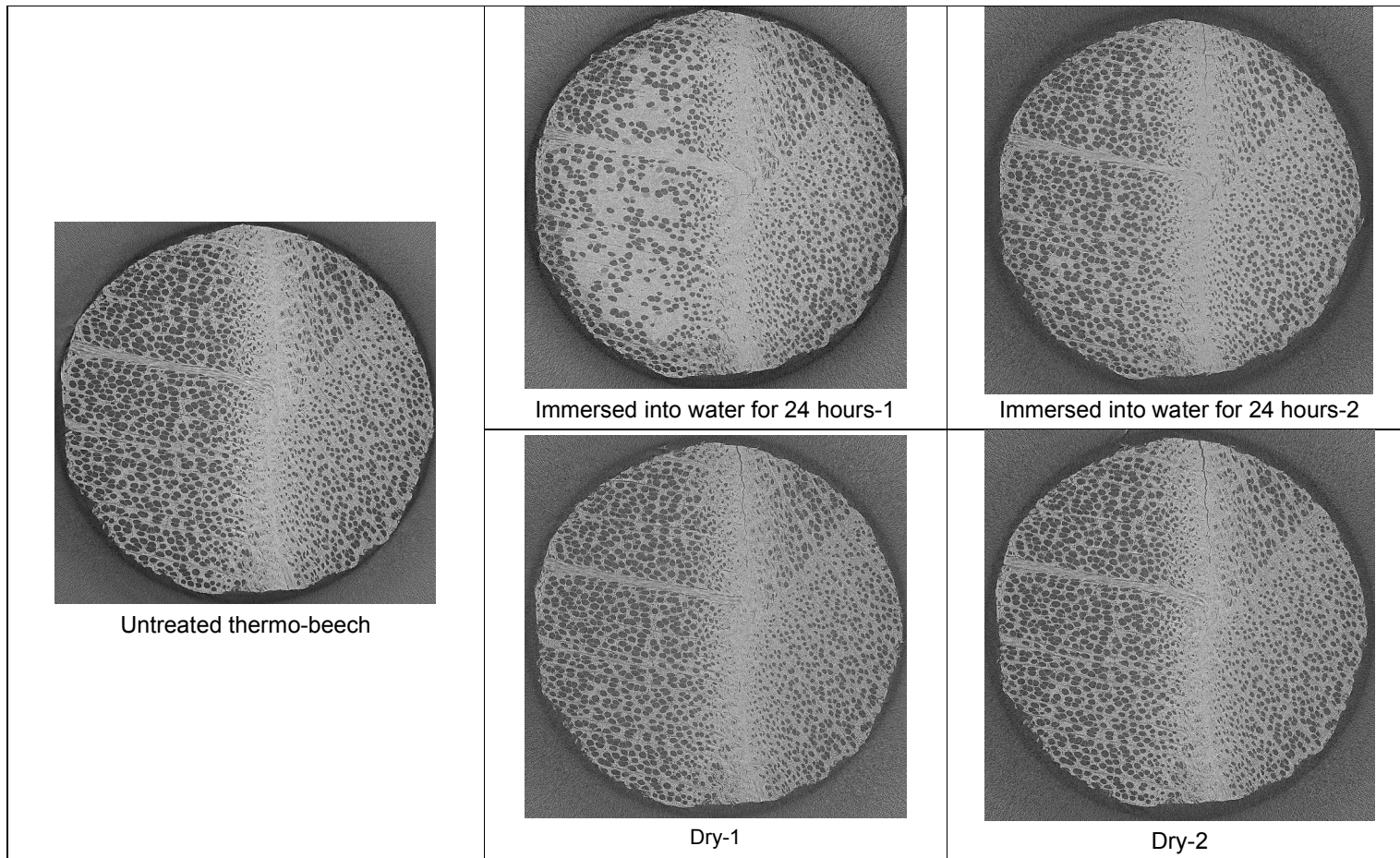
Figure 2 Tomography anatomy of welded thermo-treated beech subjected to water treatment.
