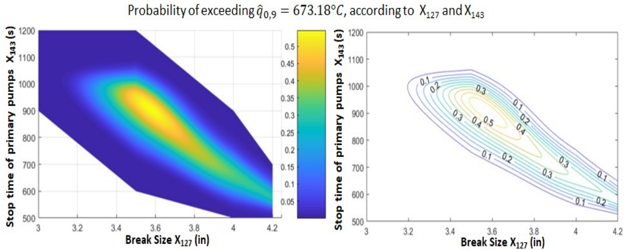
Figure 6: Estimated probability \hat{P}(X_{127}, X_{143}) of exceeding \hat{q}_{0,9} , with both surface and contour plot representations.
