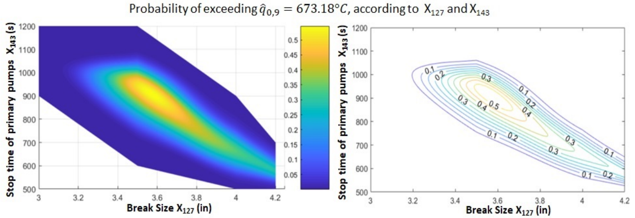
Figure 6: Estimated probability \hat{P}(X_{127}, X_{143}) of exceeding \hat{q}_{0,9} , with both surface and contour plot representations.
