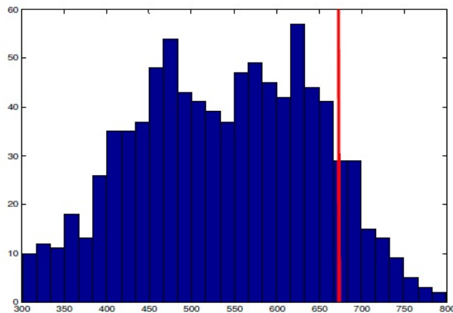
Figure 2: Histogram of the PCT from the learning sample of n = 889 simulations. The estimated 90%-quantile is indicated by the red line.
