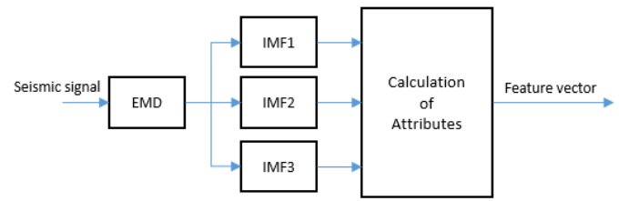
Fig. 4. Feature extraction block diagram.
