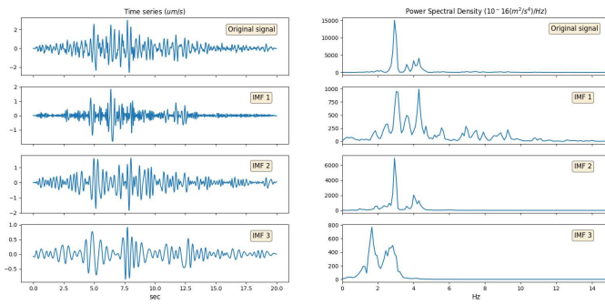
Fig. 7. A sample of an LP signal, its three selected IMFs and their PSD.
