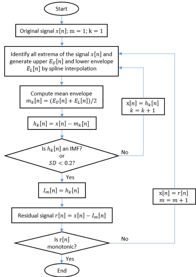
Fig. 6. Flowchart of the EMD.
