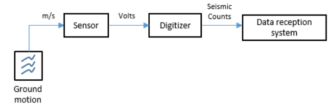
Fig. 5. Simplified block scheme of the data acquisition system from the ground motion until the reception system.
