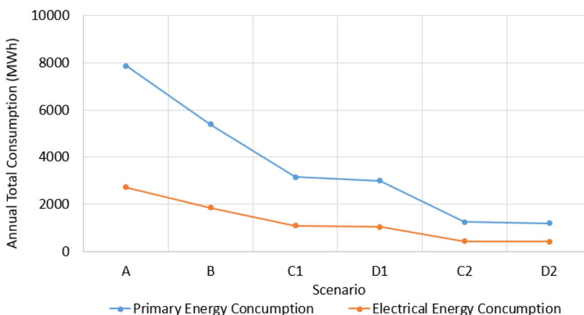
Figure 7. Total annual electrical and primary energy consumption for the examined scenarios.
