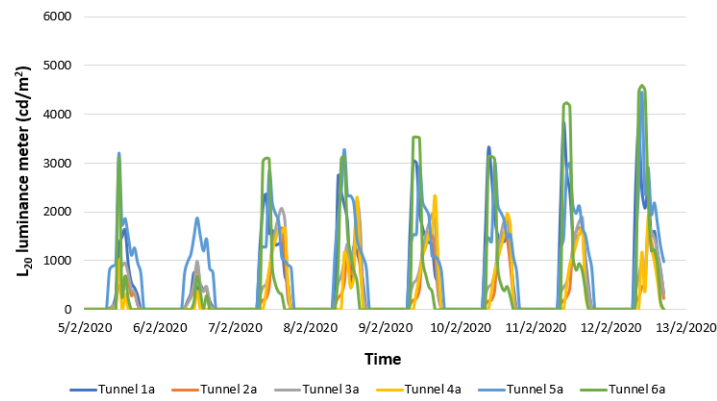
Figure 5. Signal from SCADA due to daylight variation (eight days) for the examined tunnels in the lanes leading to Athens (Tunnels 1a, 2a, 3a, 4a, 5a, and 6a).
