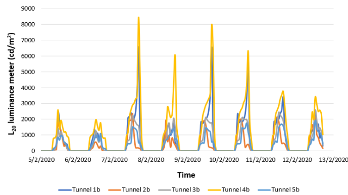
Figure 6. Signal from SCADA due to daylight variation (eight days) for the examined tunnels in the lanes leading to Lamia (Tunnels 1b, 2b, 3b, 4b, and 5b).
