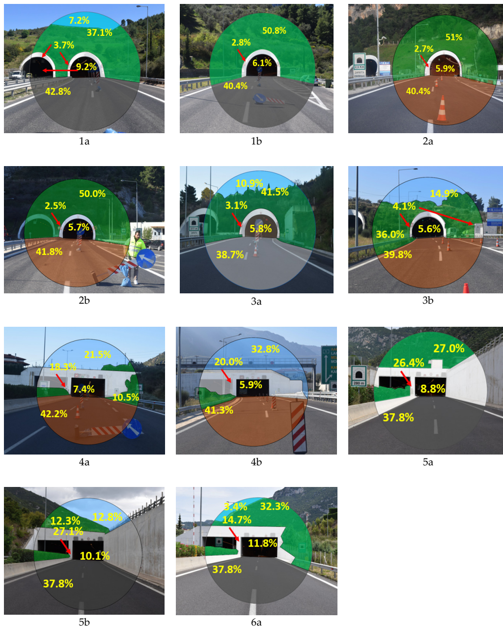
Figure 3. Photographs, taken from a point at a distance equal to the stopping distance from each of the tunnel portals in the middle of the specific motorway, presenting the parts of sky (%), road (%), surroundings (%), and portal (%) used for the calculation of the access luminance L20.
