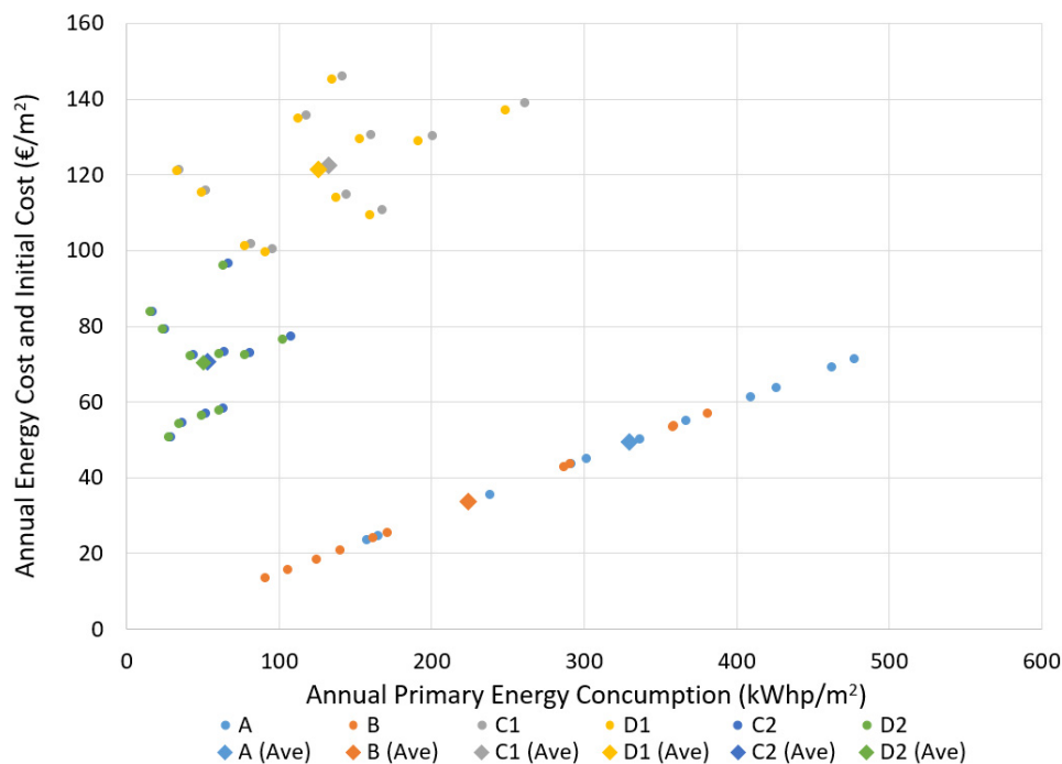
Figure 9. Annual energy cost and initial cost for LED luminaires versus the annual primary energy consumption per square meter of the entrance zone of the examined tunnels (11 tunnels in regards 6 scenarios with the corresponding average values per scenario).
