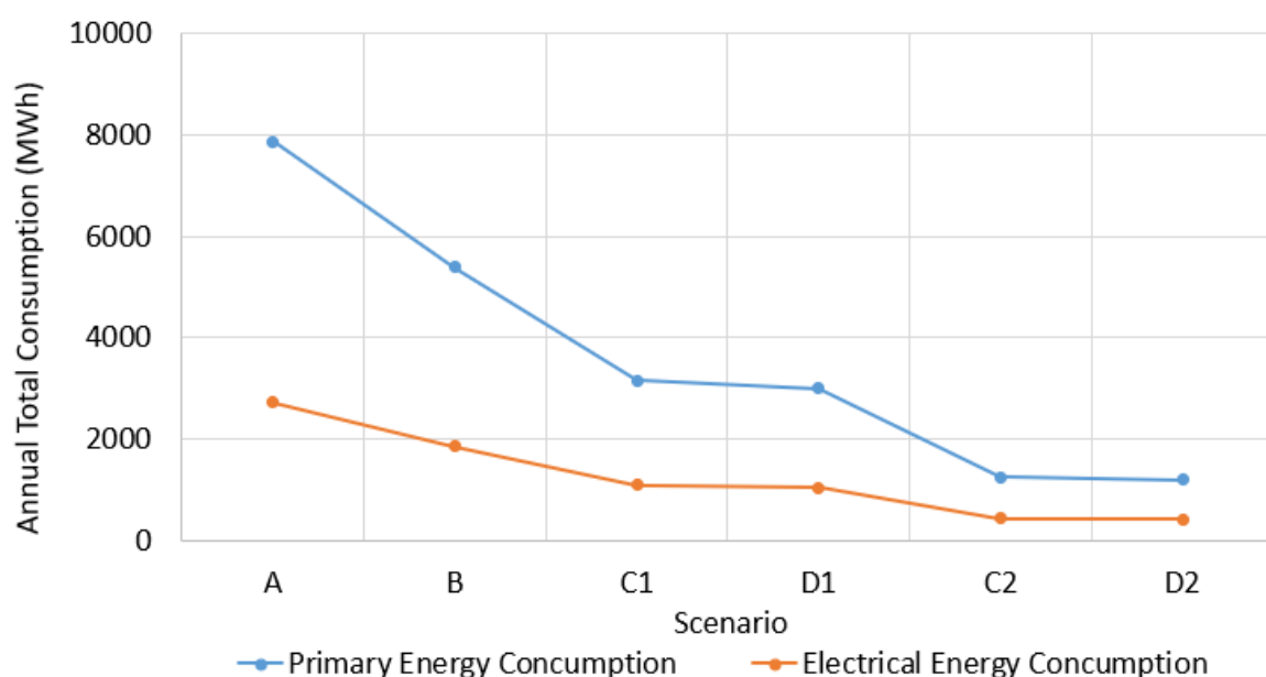
Figure 7. Total annual electrical and primary energy consumption for the examined scenarios.
