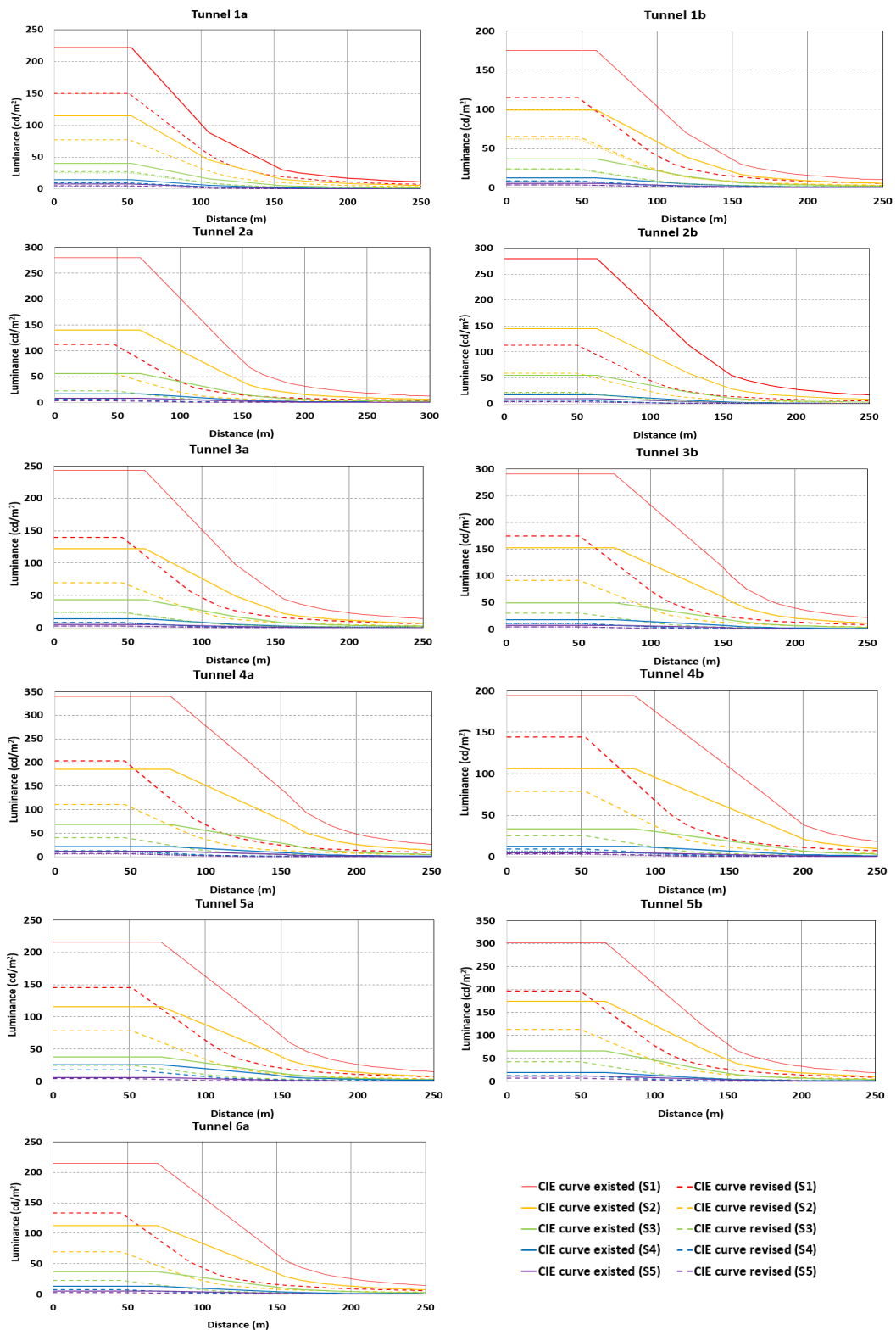
Figure 4. Luminance curves from initial design (existing lighting system) and from the traffic weighted method using the new calculated L_{th}' values, according to the Commission Internationale de l’Eclairage (CIE) for the examined tunnels.
