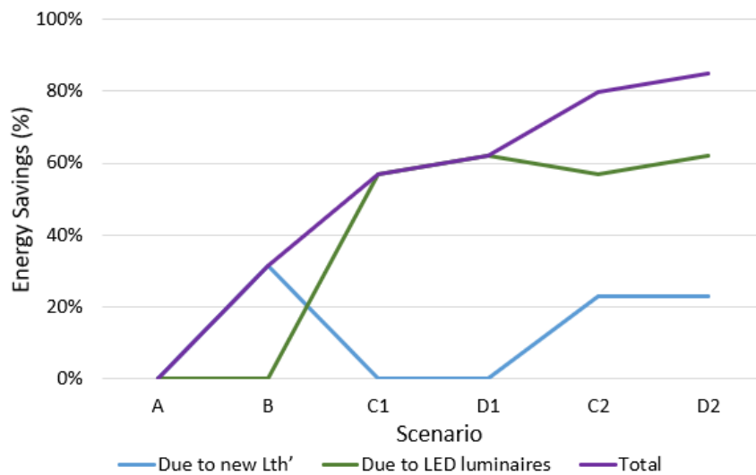
Figure 8. Breakdown of the energy savings due to the new calculated Lth' values and the retrofit of the existing luminaires with new LED luminaires for each of the examined scenarios.
