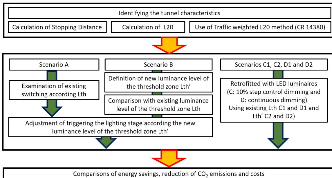
Figure 1. Diagram of the proposed methodology with the examined scenarios. Lighting Emitting Diodes (LED); threshold luminance ( L_{th} ); new corresponding threshold zone luminance ( L_{th}' ).
