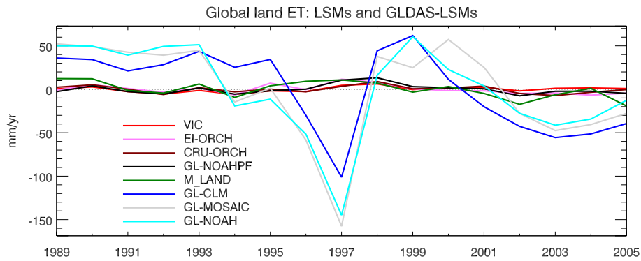
Fig. A1. Time series 1989–2005 of LSMs. In addition to the LSMs that contribute to the long-merged synthesis product, GLDAS-1 simulations from the models CLM, MOSAIC and NOAH are shown.
