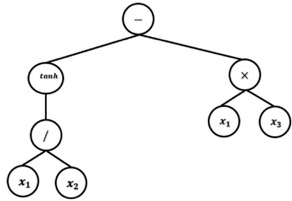
Fig. 1. A scheme of a chromosome with two genes (length of 2) and its expression.
