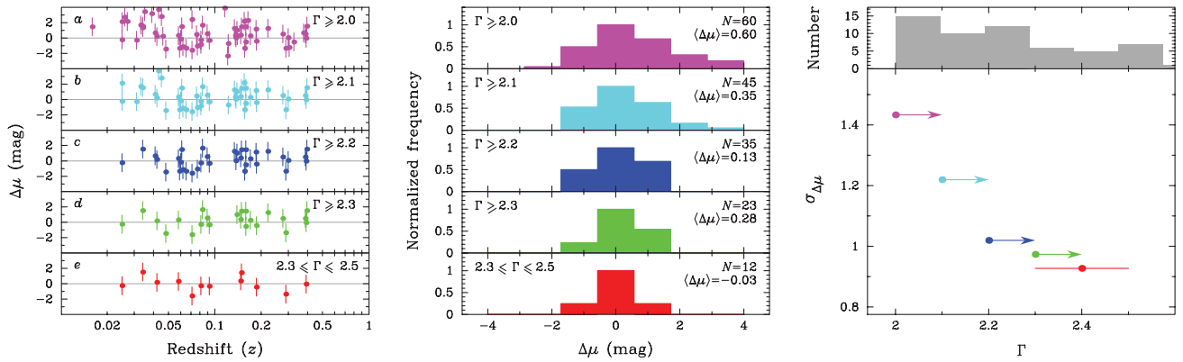
FIG. 1 (color). Left : Residuals of the SEAMBH distance modulus ( \Delta\mu = \mu_{\bullet} - \mu_L ). The error bars are taken as \Delta\mu_{\bullet} = 1.17 mag (see text for details). The assumed cosmological parameters are H_0 = 71 \text{ km s}^{-1} \text{Mpc}^{-1} , \Omega_{\Lambda} = 0.73 and \Omega_M = 0.27 . Middle : The distribution of \Delta\mu as a function of the hard x-ray (2–10 keV) photon index \Gamma . The normalized frequency is referred to fractions to the peak number of objects. N is the total number of SEAMBHs selected by \Gamma . Right : scatter of the \Delta\mu distributions with \Gamma (bottom) and the distribution of \Gamma for the sample of SEAMBH candidates. The dependence of the dispersion in the residuals as a function of \Gamma shows a systematic decrease and tends to \sigma_{\Delta\mu}^{\text{min}} , indicating the efficacy of the selection as standard candles.
