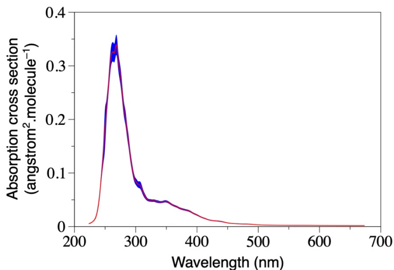
Figure 6. Simulated absorption spectrum of 2o resulting from S_0 \rightarrow S_1(1^1B_g) , S_0 \rightarrow S_2(1^1B_u) , S_0 \rightarrow S_3(2^1B_g) , S_0 \rightarrow S_4(1^1A_u) and S_0 \rightarrow S_5(2^1B_u) electronic transitions using the NE approach. The blue area indicates the error in the absorption cross section due to the statistical sampling.
