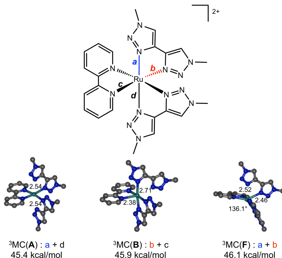
Figure 5: Examples of classical (trans-elongated, A/B) and flattened (cis-elongated, F) ^{3}\text{MC} minima with remarkable distances along the most elongated bonds ( a+d , b+c or a+b ) and angles. Electronic energies with respect to that of the ground state [87].
