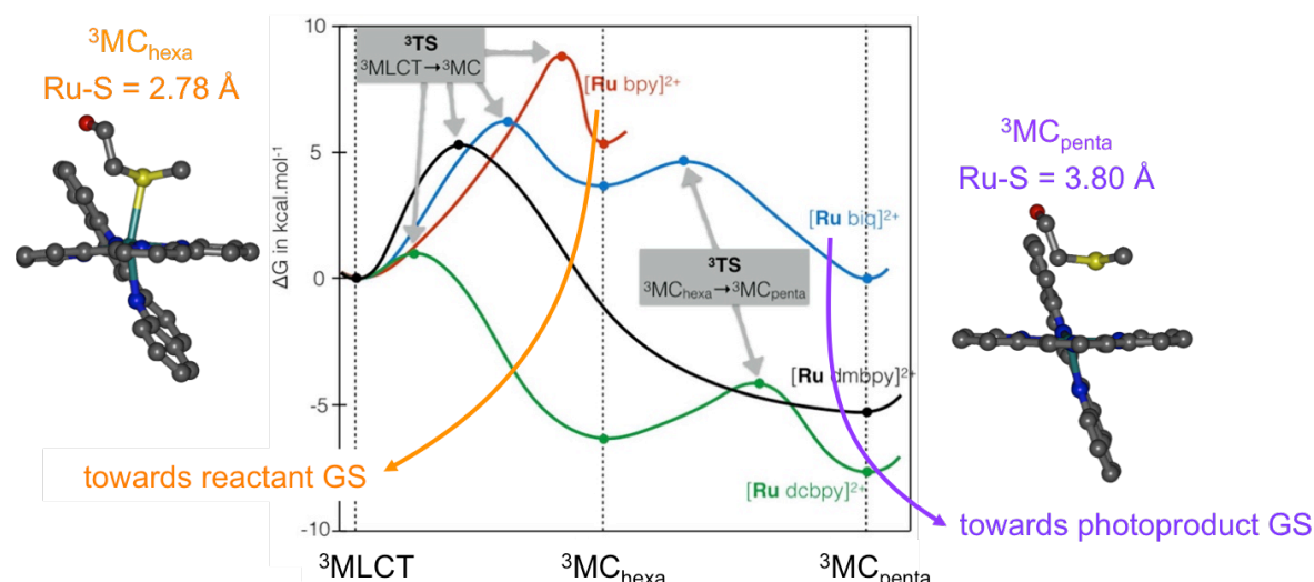
Scheme 3: Triplet free energy profiles for the bpy (red), dcbpy (green), biq (blue) and dmbpy (black) complexes in water at 298 K ( ^3 MLCT states aligned for comparison purposes). The preferential roles assigned to ^3 MC _{hexa} (geminate recombination towards starting material, orange arrow) and ^3 MC _{penta} (evolution towards photoproduct, purple arrow) are schematized through crossings with the relevant singlet PES. Illustration with the biq ligand showing the chemical structure and Ru-S distance in the ^3 MC states proposed to play two distinct roles [67].
