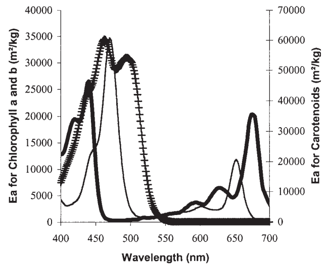
Figure 2. Data bank of in vivo absorption coefficients of pure pigments (— chlorophyll a, - - - chlorophyll b, + + + carotenoids). Data are from Bidigare et al. (1990).
