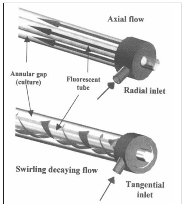
Figure 2. Axial and swirling flows.
