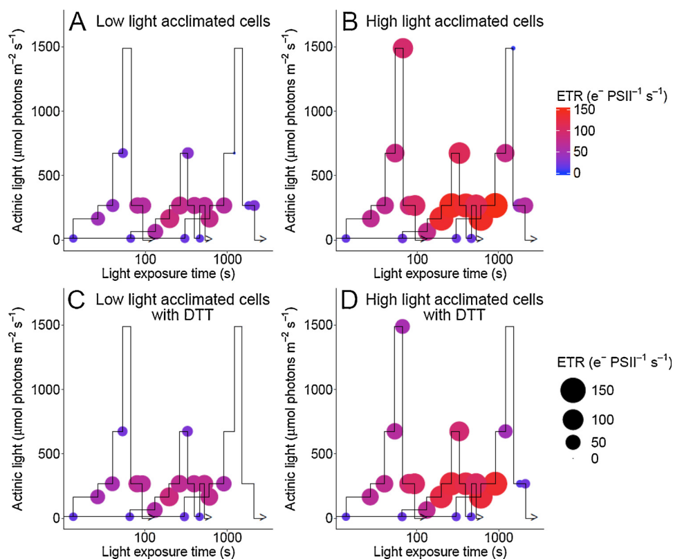
Fig. 6. Actinic light levels (black trace) plotted vs. duration of light exposures PSII ETR ( e^-PSII^{-1} s^{-1} ) in C. vulgaris control cultures (A and B) and in presence with DTT (C and D) shown by symbol size and colour scale. Cultures were grown at 30 \mu mol m^{-2} s^{-1} (Low light, A and C) and 330 \mu mol m^{-2} s^{-1} (High light, B and D). PSII ETR was estimated according to Eqn. 5.
