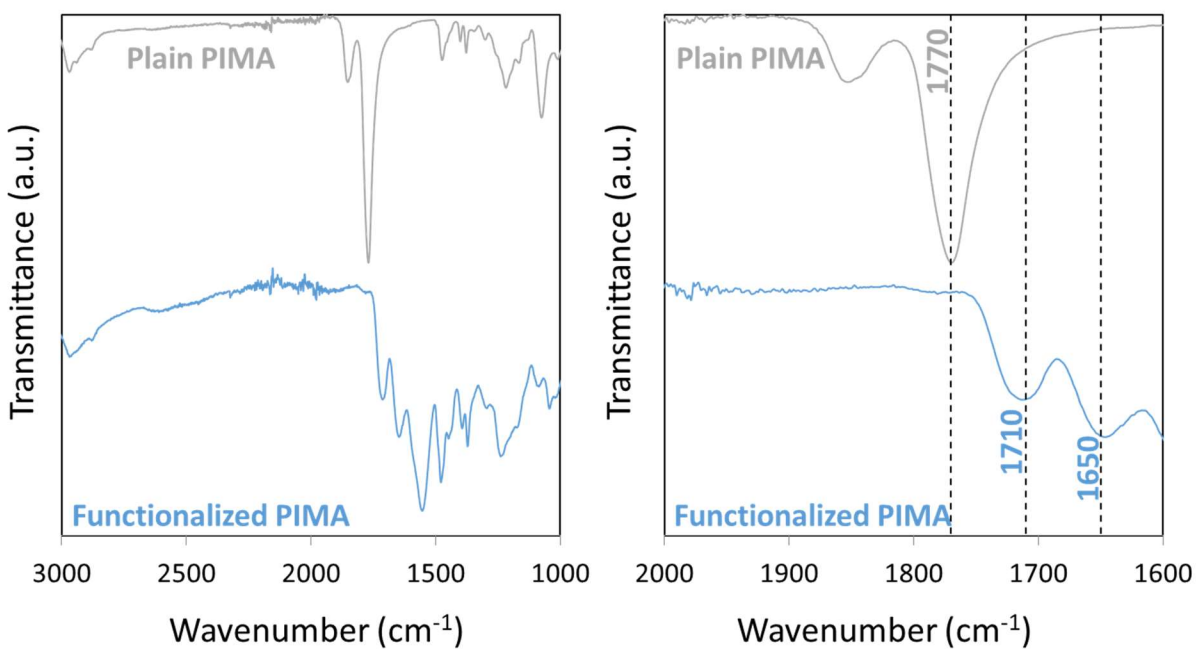
Figure 1. FTIR spectra of the as-shipped (grey) and functionalized PIMA polymer (blue). The full spectrum is plotted on the left, while a narrower region is plotted on the right to highlight the wavenumbers of interest.
