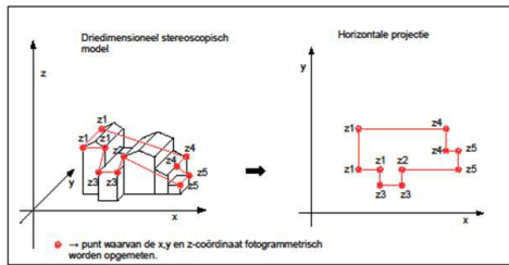
Figure 8 3D characteristics of buildings captured in the 3D modelling process by IGN, Belgium
