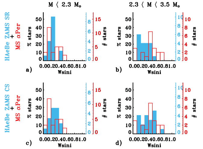
Figure 7. W \sin i histograms of the H AeBe projected on the ZAMS (blue field bars) assuming an SR (top) or assuming a CS (bottom), and of the MS stars from the catalogue \alpha Per (red empty bars) of Prosser (1992), for two different mass ranges M < 2.3 M_{\odot} and 2.3 < M < 3.5 M_{\odot} .
