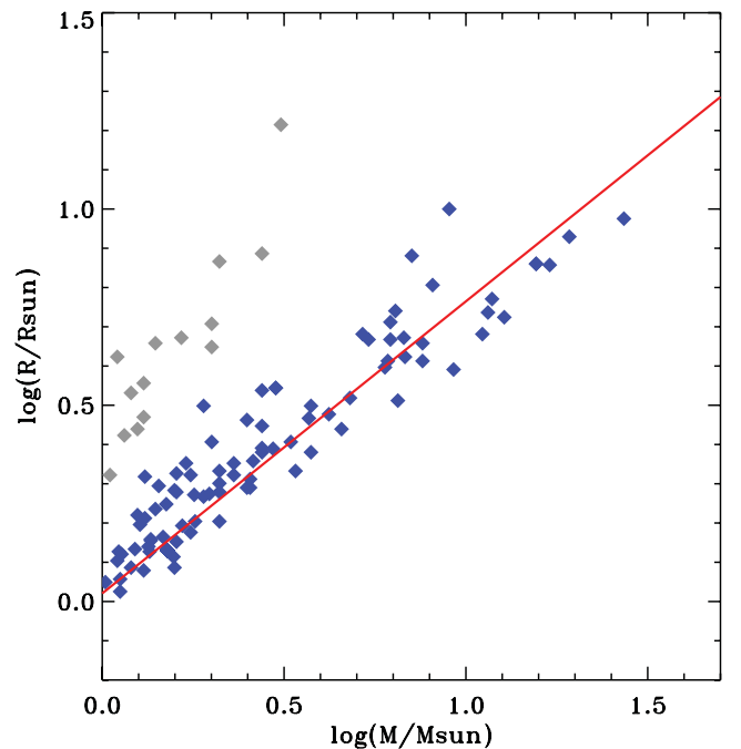
Figure B1. Radii as a function of masses for the stars of the catalogue of Svechnikov & Bessonova (1984). The linear fit is overplotted. The rejected data points are plotted in light grey.
