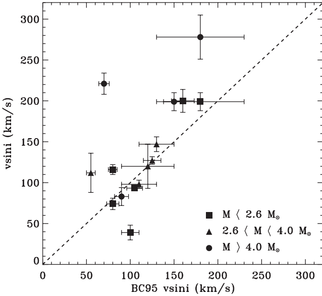
Figure 8. v \sin i of this work compared to v \sin i of BC95, for three mass ranges: M < 2.6 M_{\odot} (squares), 2.6 < M < 4.0 M_{\odot} (triangles) and M > 4 M_{\odot} (dots). The dashed line is the first bisector.
