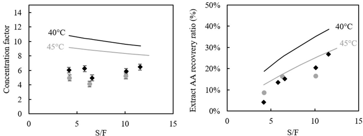
Fig. 4. Comparison between experiments (black dots: 40 °C and grey dots: 45 °C) and modelling (continuous lines) for one theoretical stage at 40 °C (black lines) and 45 °C (grey lines). Influence of S/F on the recovery ratio of AA and concentration factor (10 MPa, F=0.48 kg/h, 5 % w/w AA).
