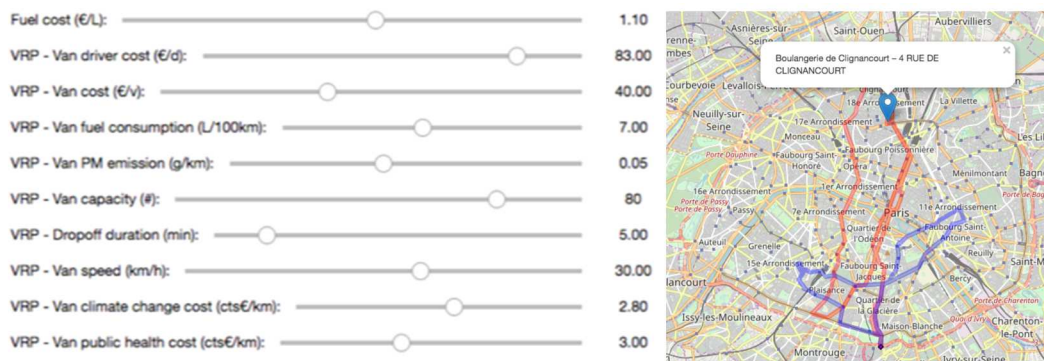
Fig. 2. On the left, simulator parameters are easily customizable using sliders. On the right, vehicles itineraries are plotted on a real map.
