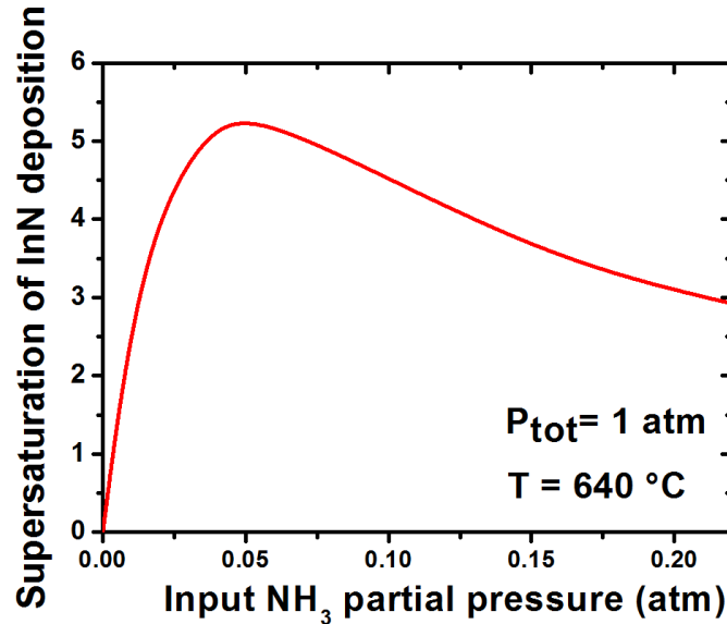
Figure 3: Plot of the supersaturation parameter for InN deposition as a function of the input NH 3 partial pressure. P_{\text{tot}} is the total pressure in the reactor. The supersaturation in the vapor phase to promote InN deposition decreases at higher P_{\text{NH}_3}^0 .
