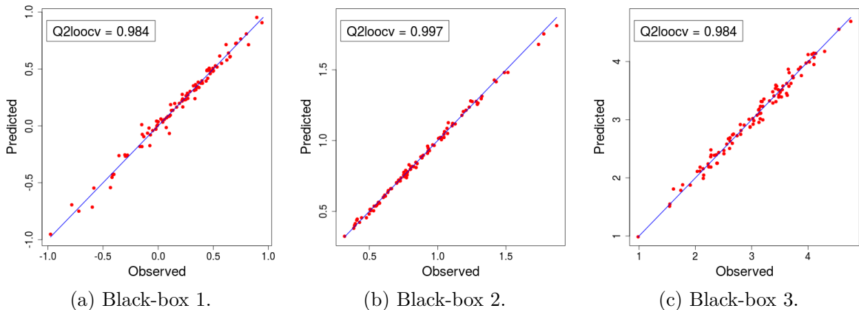
Figure 6: Calibration plot for selected models.
