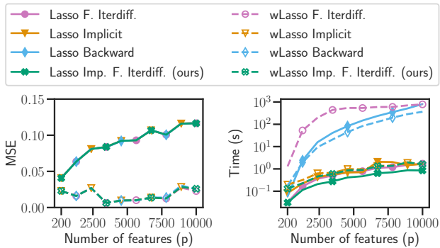
Figure 4. Lasso vs wLasso. Estimation Mean Squared Error (left) and running (right) of competitors as a function of the number of features for the weighted Lasso and Lasso models.
