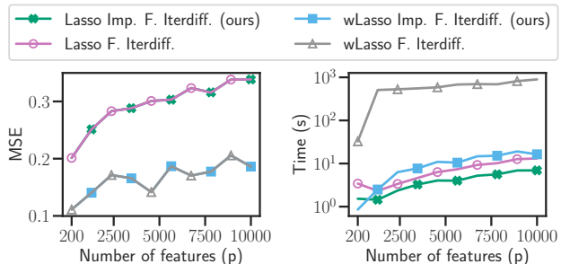
Figure 4. Lasso vs wLasso. Estimation Mean Squared Error (left) and running (right) of competitors as a function of the number of features for the weighted Lasso and Lasso models.
