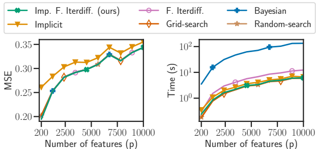
Figure 3. Lasso: estimation performance. Estimation Mean Squared Error (left) and running time (right) as a function of the number of features for the Lasso model.
