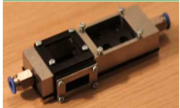
Fig. 3. Top: functional sketch of the full sensor cell bottom. The mylar membrane is in the bottom left part while, in the upper right part, four commercial sensors are installed. Bottom: corresponding realized cell
