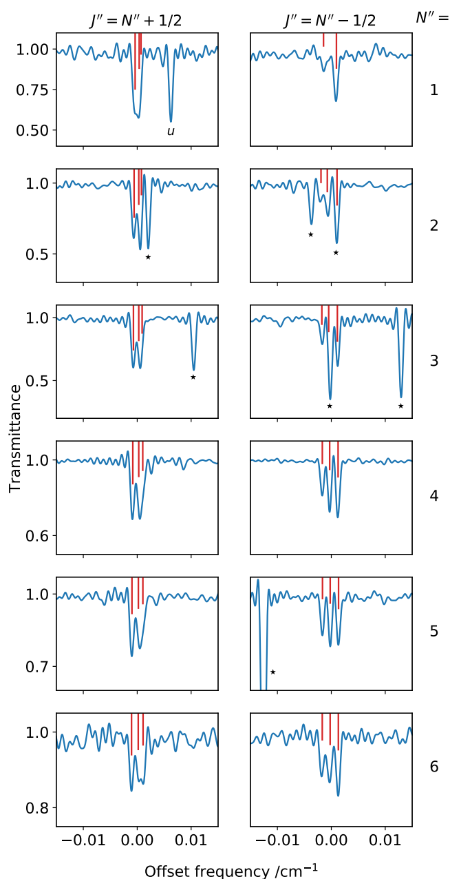
Fig. 3. Observation on the FIR spectrum of the hyperfine structure due to the nuclear spin of the N atom in NHD for the b -type \nu R(1) branch with K''_a + K''_c - N'' = 0 . Frequencies are reported as the offset frequencies from the predicted transition when no hyperfine structure is taken into account and span the 68\text{--}188\text{ cm}^{-1} range (see the supplementary material for the numerical values). Predicted frequency of each component (neglecting the H and D hyperfine splittings) is indicated by red sticks (intensity in arbitrary units). Transitions labelled with “*” symbol are still present with the discharge off and most likely arise from \text{ND}_3 ; the line labelled with a “u” remains unassigned.
