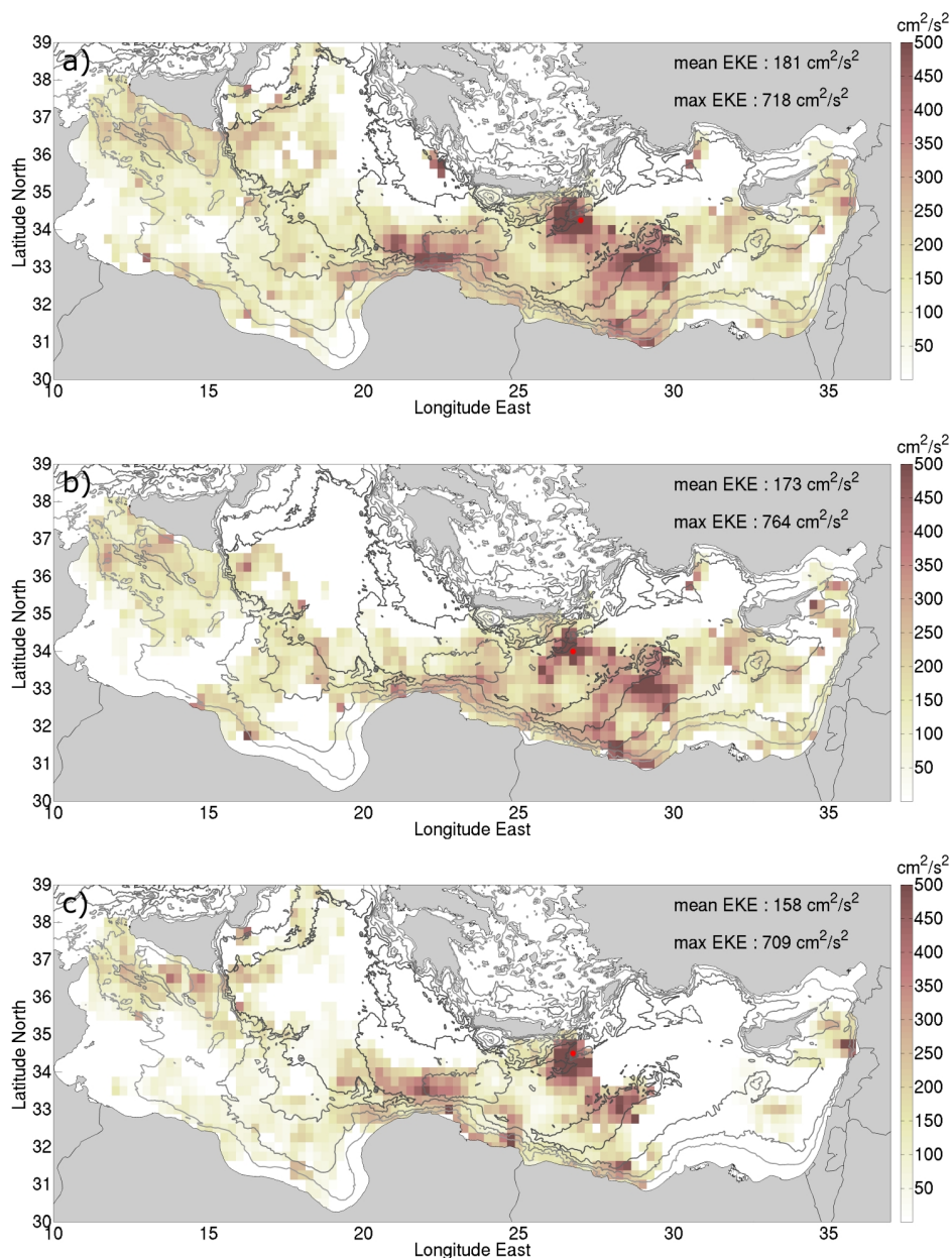
Fig. 11. EKE (saturated at 500 \text{ cm}^2/\text{s}^2 ) for the whole dataset (a), for the extended winter (b) and for the extended summer (c). Data are grouped into 0.5^\circ \times 0.5^\circ bins overlapped by 50% and results for bins with less than 10 observations and 2 different drifters are not plotted. The undrogued observations with a speed ratio (wind-induced slip/drifter speed) larger than 50% were not considered in the computation. The 200 m, 1000 m, 2000 m and 3000 m isobaths are represented in grey tones. The red dot indicate the absolute maxima.
