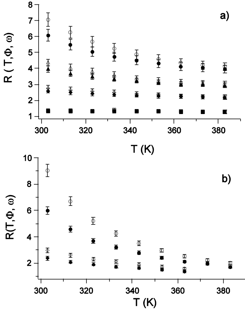
Figure 5 : Temperature and frequency dependence of the reinforcement R(T, \Phi, \omega) for T > T_g + 50K and two frequencies \omega = 1Hz (open) and \omega = 0.01Hz (filled). a) TPM_I samples; ( \square ) : \Phi = 0.07 ; ( \diamond ) : \Phi = 0.12 ; ( \triangle ) : \Phi = 0.15 ; ( \circ ) : \Phi = 0.18 . b) ACS samples ( \diamond ) : \Phi = 0.12 ; ( \circ ) : \Phi = 0.18 .
