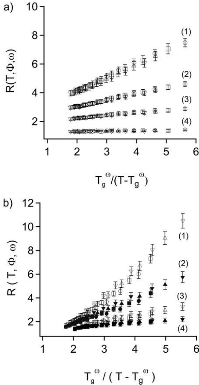
Figure 7 : a) Variation of the reinforcement R versus T_g^\omega/(T-T_g^\omega) for different frequencies and different silica concentrations for the TPM_I sample : (○) : \omega=10 Hz, (□): \omega=1 Hz, (△) : \omega=0.1 Hz, (▽) : \omega=0.01 Hz. (1) : \Phi=0.18 ; (2) : \Phi=0.15 ; (3) : \Phi=0.12 ; (4) : \Phi=0.08 . b) Variation of the reinforcement R versus T_g^\omega/(T-T_g^\omega) for different frequencies and different silica concentrations for the ACS sample : for (1) : \Phi=0.18 and (3) : \Phi=0.12 (○) : \omega=10 Hz, (□): \omega=1 Hz, (△) : \omega=0.1 Hz, (▽) : \omega=0.01 Hz . For (2) : \Phi=0.15 and (4) : \Phi=0.09 , (●) : \omega=10 Hz, (■) : \omega=1 Hz, (▲) : \omega=0.1 Hz, (▼): \omega=0.01 Hz.
