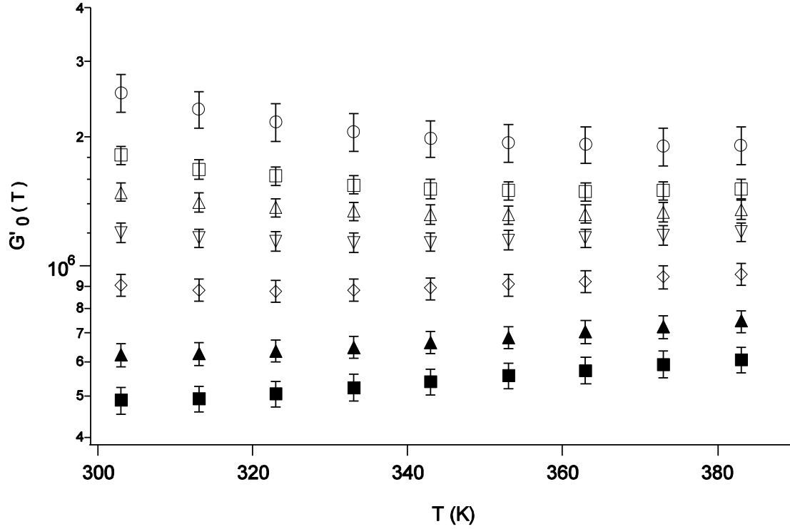
Figure 3 : Temperature dependence of the real part of the shear modulus G'(T) for TPM_I samples having varying silica concentration for temperatures T higher than T_g^\circ + 50K . (■) : \Phi = 0.07 ; (▲): \Phi = 0.09 ; (◇): \Phi = 0.12 ; (▽): \Phi = 0.14 ; (△): \Phi = 0.15 ; (□): \Phi = 0.16 ; (○): \Phi = 0.18 .
