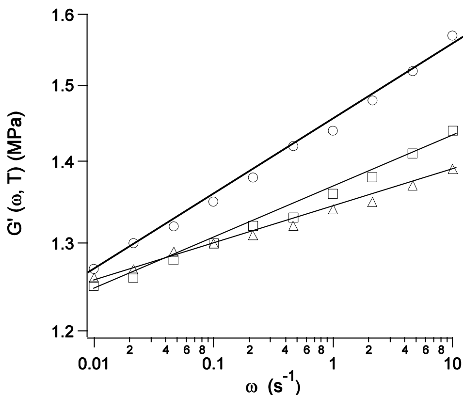
Figure 4 : Variation of the frequency dependence of the real part of the shear modulus with the temperature for a filled TPM_I elastomer with a silica volume fraction \Phi=0.16 . (○): T = 323 K, (□) : T = 343 K, (△) : T = 363 K The straight lines are eyes guide showing the variation of the temperature dependence of the slope of G'(\omega) .
