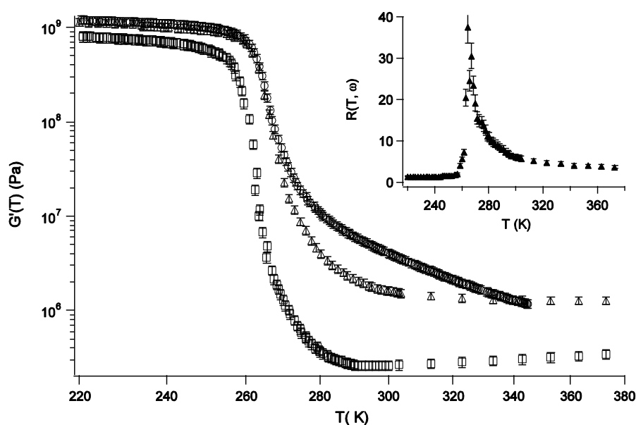
Figure 2 : Temperature dependence of the real part of the shear modulus G'(T) in the linear regime for different silica concentrations : ( \square ) : \Phi=0 , ( \triangle ) : \Phi=0.16 TPM_I sample, ( \circ ) : \Phi=0.18 ACS sample. Insert: Temperature dependence of the reinforcement for the TPM_I sample containing a silica volume fraction \Phi=0.16 .
