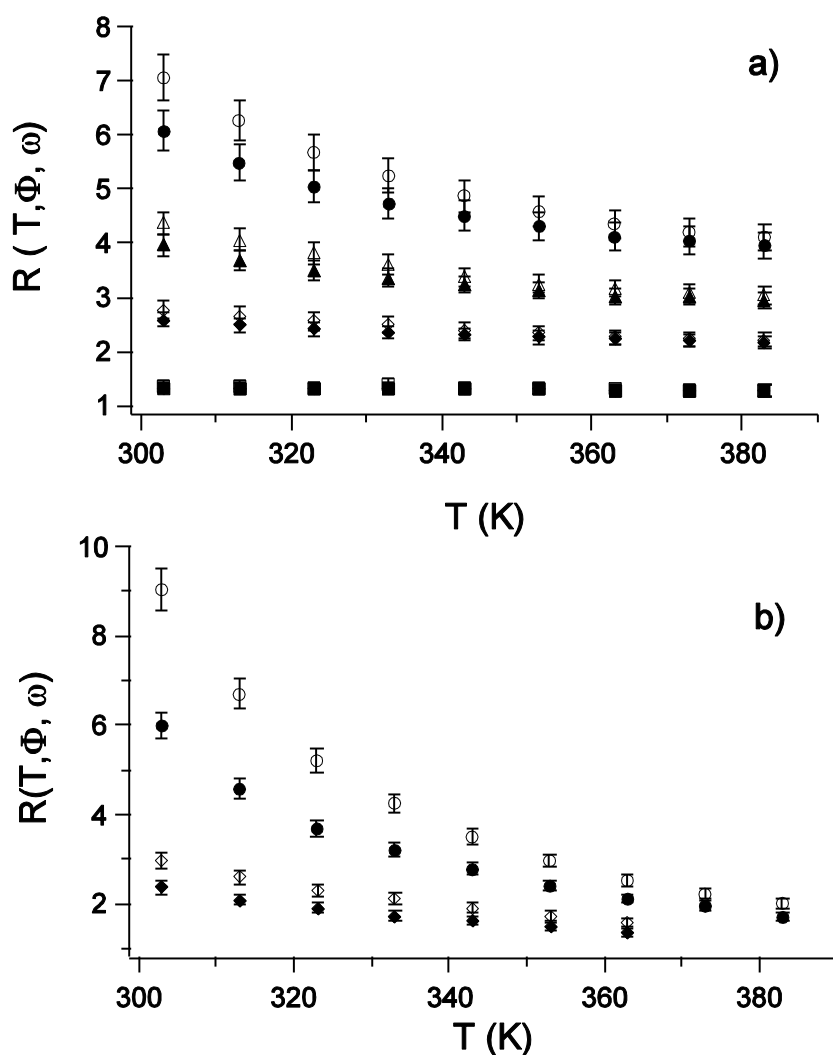
Figure 5 : Temperature and frequency dependence of the reinforcement R(T, \Phi, \omega) for T > T_g + 50K and two frequencies \omega = 1 Hz (open) and \omega = 0.01 Hz (filled). a) TPM_I samples; ( \square ) : \Phi = 0.07 ; ( \diamond ) : \Phi = 0.12 ; ( \triangle ) : \Phi = 0.15 ; ( \circ ) : \Phi = 0.18 . b) ACS samples ( \diamond ) : \Phi = 0.12 ; ( \circ ) : \Phi = 0.18 .
