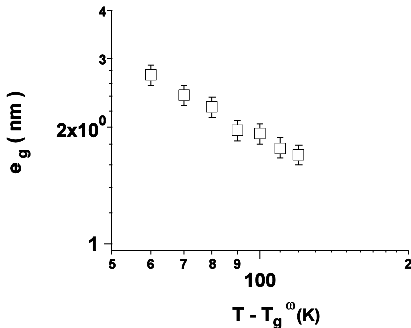
Figure 1: Variation of the thickness e_g of the glassy shell around the particles versus temperature. Data from N.M.R measurements : (□)
