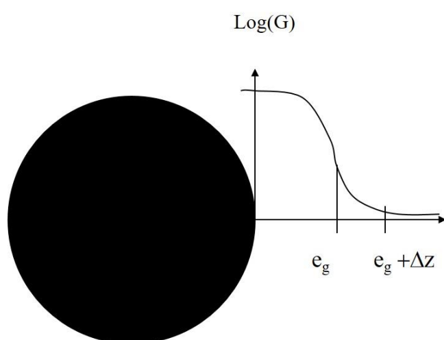
Figure 6 : Schematic representation of the variation of the modulus of the polymer chains near a particle (in black) versus the distance to the particle surface. For z < e_g , the polymer is in a glassy state G=G_{\text{glass}} . At z > e_g + \Delta z G=G_N where G_N is the plateau modulus of the elastomer matrix.
