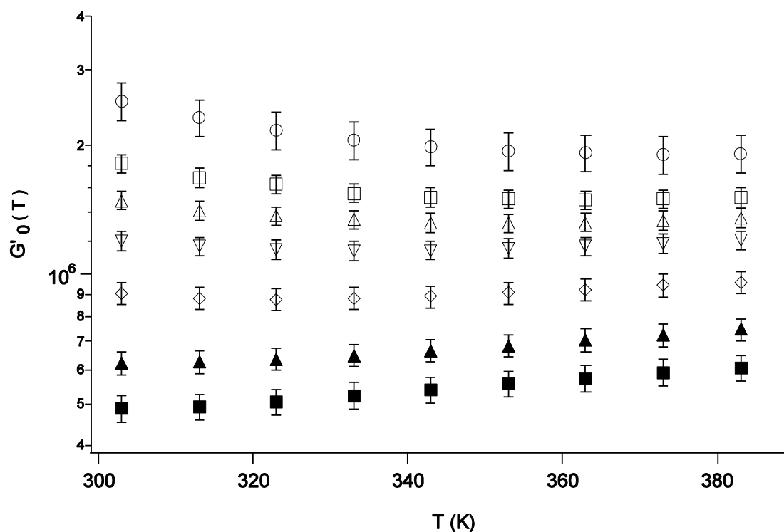
Figure 3 : Temperature dependence of the real part of the shear modulus G'(T) for TPM_I samples having varying silica concentration for temperatures T higher than T_g^0 + 50K . (■) : \Phi = 0.07 ; (▲): \Phi = 0.09 ; (◇): \Phi = 0.12 ; (▽): \Phi = 0.14 ; (△): \Phi = 0.15 ; (□): \Phi = 0.16 ; (○): \Phi = 0.18 .
