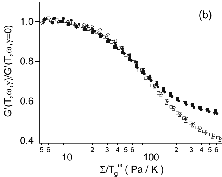
Figure 5: Master curves showing the dependence of the normalized real part of the shear dynamical modulus G'(T, \omega, \gamma)/G'(T, \omega, \gamma=0) on the deformation \gamma at constant T_g^\omega/(T-T_g^\omega) . (a) : MCS_II sample with \Phi=0.214 . T_g^\omega/(T-T_g^\omega) = 3.783 : (○) \omega = 0.01\text{Hz} and T=308.5\text{K} , (□) \omega = 0.1\text{Hz} and T=314\text{K} , (△) \omega = 1\text{Hz} and T=319.5\text{K} , (▽) \omega = 10\text{ Hz} and T=325\text{K} . T_g^\omega/(T-T_g^\omega) = 2.464 : (●) \omega = 0.01\text{Hz} and T=343\text{ K} , (■) \omega = 0.1\text{Hz} and T=348.5\text{ K} , (▲) \omega = 1\text{Hz} and T=354\text{ K} , (▼) \omega = 10\text{ Hz} and T=359.5\text{ K} . (b) : ACS sample with \Phi=0.18 . T_g^\omega/(T-T_g^\omega) = 3.783 : (○) \omega = 0.01\text{Hz} and T=308.5\text{K} , (□) \omega = 0.1\text{Hz} and T=314\text{K} , (△) \omega = 1\text{Hz} and T=319.5\text{K} , (▽) \omega = 10\text{ Hz} and T=325\text{K} . T_g^\omega/(T-T_g^\omega) = 2.464 : (●) \omega = 0.01\text{Hz} and T=343\text{ K} , (■) \omega = 0.1\text{Hz} and T=348.5\text{ K} , (▲) \omega = 1\text{Hz} and T=354\text{ K} , (▼) \omega = 10\text{ Hz} and T=359.5\text{ K} .
