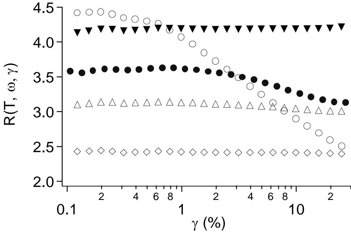
Figure 2 : Variation of the reinforcement R(T, \omega, \gamma) of MCS_I, TPM_VI and TPM_III samples versus deformation at T=303K : (▼) : MCS_I with \Phi=0.24 ; (◇) TPM_III with \Phi=0.18 ; (△) TPM_VI with \Phi=0.18 ; (●) MCS_II with \Phi=0.15 , (○) ACS with \Phi=0.15 .
