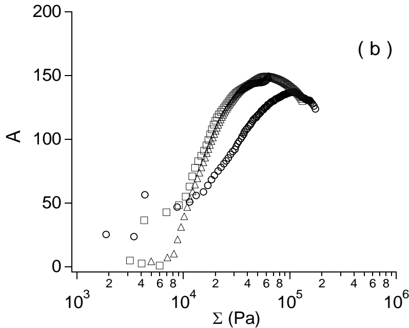
Figure 6: Comparison of the effect of macroscopic stress and temperature on the value of the reinforcement of a MCS_II sample having the silica volume fraction of 0.214. (a) The curves showing the temperature dependence of the reinforcement R_T versus K(T-T_0) are plotted in solid lines ( K_y=1 \text{ MPa K}^{-1} ). The variation of the reinforcement with the macroscopic stress \Sigma are plotted in markers : T = 303\text{K} ( \circ ), T = 323\text{K} ( \square ) and T = 343\text{K} ( \triangle ). (b) Variation of the parameter A with the macroscopic stress \Sigma for three temperatures : T=303\text{K} ( \circ ), T= 323\text{K} ( \square ) and T= 343\text{K} ( \triangle ). The arrows on figure 6-a point out the position of the maximum of A observed on the figure 6-b.
