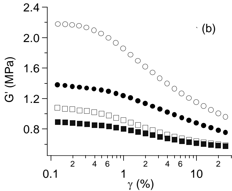
Figure 1 : Variation of the real part of the shear modulus G' versus the deformation \gamma . (a) MCS_II samples \Phi= 0.21 : ( \circ ) \omega = 0.1\text{Hz} and T=303\text{ K} , ( \square ) \omega = 0.1\text{Hz} and T=343\text{K} , ( \triangle ) \omega = 0.01\text{ Hz} and T=303\text{K} . \Phi= 0.15 : ( \bullet ) \omega = 0.1\text{Hz} and T=303\text{K} , ( \blacktriangle ) \omega = 10\text{ Hz} and T=303\text{K} . (b) ACS samples \Phi= 0.18 : ( \circ ) \omega = 0.1\text{Hz} and T=303\text{K} , ( \square ) \omega = 0.1\text{Hz} and T=343\text{K} ,. \Phi= 0.15 : ( \bullet ) \omega = 0.1\text{Hz} and T=303\text{K} , ( \blacksquare ) \omega = 0.1\text{Hz} and T=343\text{K} .
