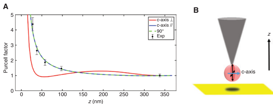
Figure 6: Modification of the Purcell factor as a function of z , (A) red and blue lines are extreme orientations of the c -axis and green dotted line corresponds to the one fitting the experimental results, black dots for experimental results, (B) scheme of the NC at the end of the tip corresponding to the measurements, c -axis parallel to the surface.
