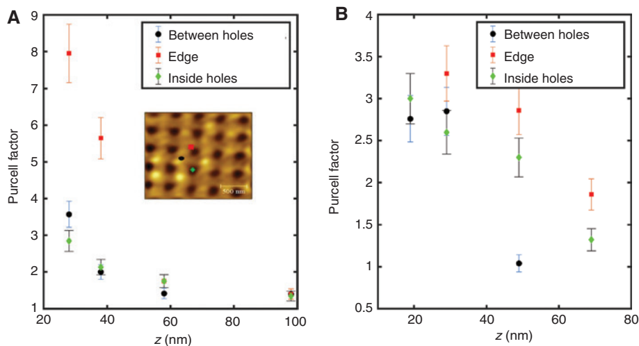
Figure 8: The Purcell factors measured at three positions for different altitudes z and for both active probes. (A) Purcell factors as a function of z for NC_1 with a c-axis parallel to the surface for three positions on the array shown on the atomic force microscopic image and (B) for NC_2 with a 40^\circ c-axis angle.
