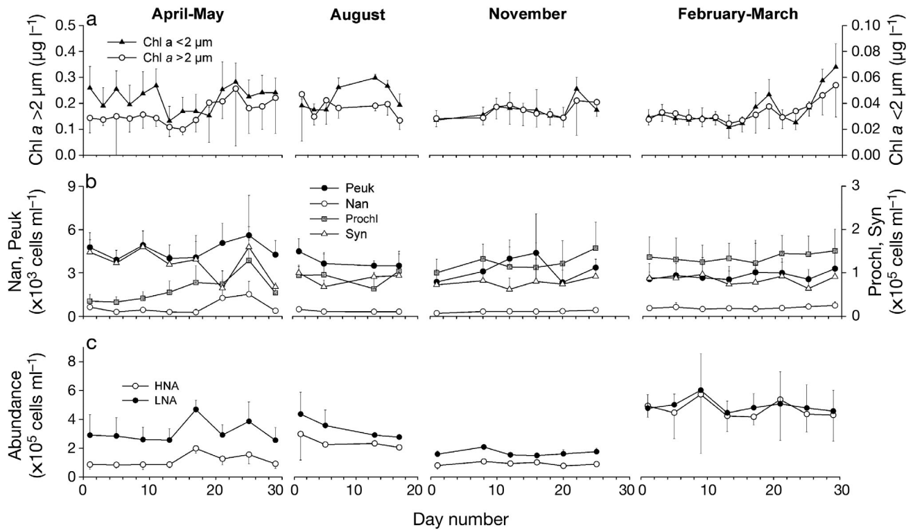
Fig. 5. Day-to-day variation in the (a) concentrations of chl a > 2 µm (left scale) and < 2 µm (right scale), (b) abundances of nanophytoplankton (Nan) & picoeukaryotes (Peuk) (left scale) and Prochlorococcus (Prochl) & Synechococcus (Syn) (right scale), and (c) abundances of high-nucleic acid (HNA) & low-nucleic acid (LNA) bacteria at 5 m depth during the 4 surveys (April–May 2007, August 2007, November 2007 and February–March 2008). Data are means ( \pm SD) of measurements at the 12 lagoon stations
