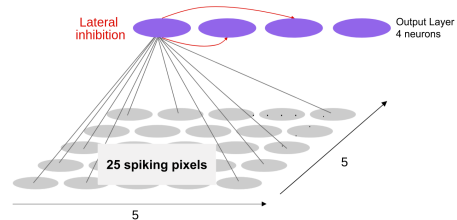
Figure 2: Topological overview of the network.
