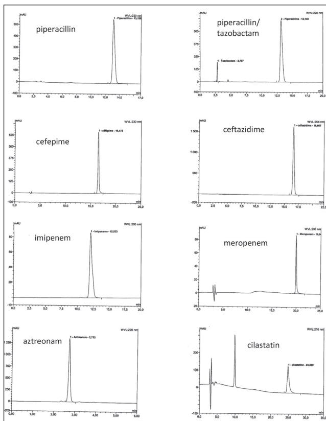
Fig. 1: Representative chromatograms
